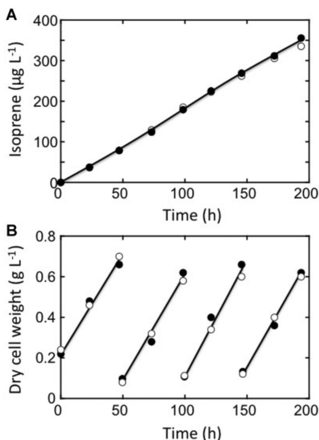
Figure 9. Continuous growth for biomass and isoprene production in a gaseous/aqueous two-phase bioreactor. Sk/spS transformant cultures were administered 500 mL of 100% CO 2 approximately every 24 h to maintain photoautotrophic growth while the bioreactor was sealed for isoprene accumulation. Cultures were also diluted with fresh growth media every 48 h to an OD 730 nm = 0.5 (~0.2 g dw L -1 ) in order to maintain cells in the actively dividing stage. A: Isoprene hydrocarbons accumulated over the time course of the experiment. B: Culture dry cell weight as a function of time during continuous growth in the bioreactor. Dilutions of the culture were implemented at 48, 96, and 144 h. Results shown are for two different Sk/spS transformant lines.
