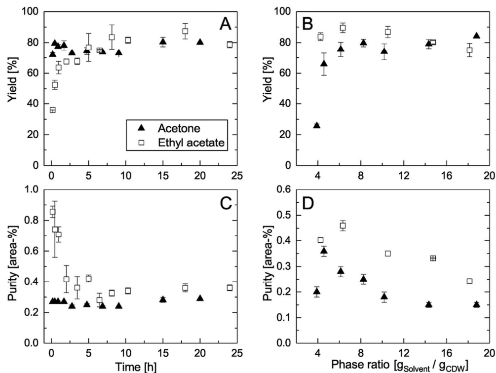
Figure 6. Comparison of betulinic acid yield (A, B) and purity (C, D) obtained with acetone and ethyl acetate as extractant in dependence on extraction time (phase ratio 10 g Solvent /g CDW , at 25 °C) and phase ratio at 25°C.
