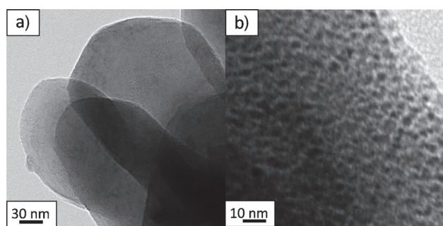
Figure 1. a) HR-TEM images of 3.2 wt% Cu-HT. b) Higher magnification image of Cu-HT catalyst reveals the size and distribution of the Cu nanoparticles.
