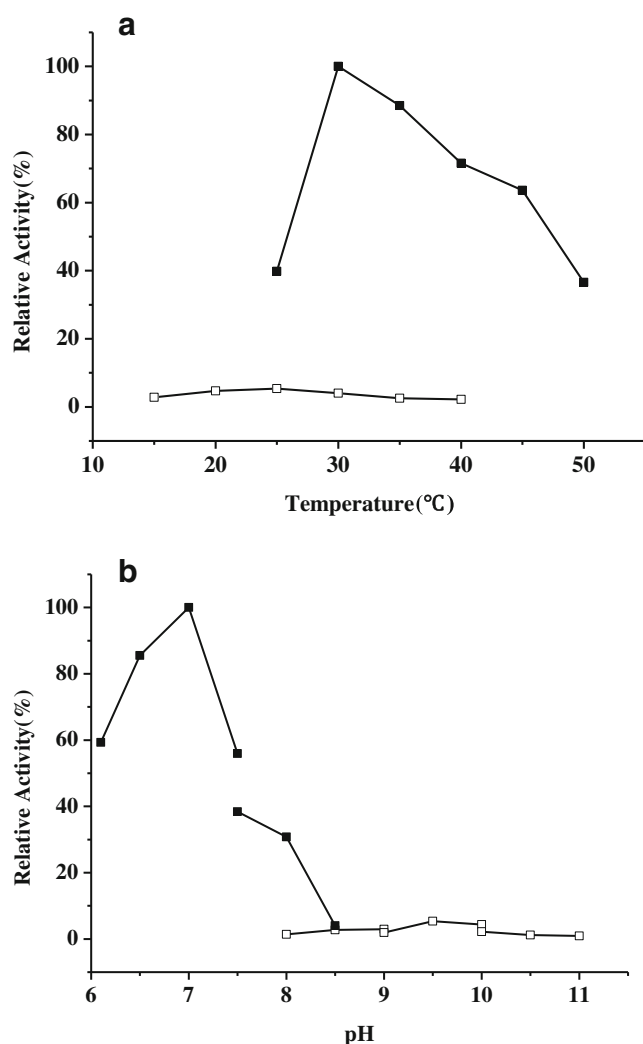
Fig. 3 Effect of temperature ( a ) and pH ( b ) on the activities of ReADR. The relative activity of 100 % represents 9.16 U/mg for diacetyl reduction at 30 °C and pH 7.0. Solid symbols reduction, empty symbols oxidation
