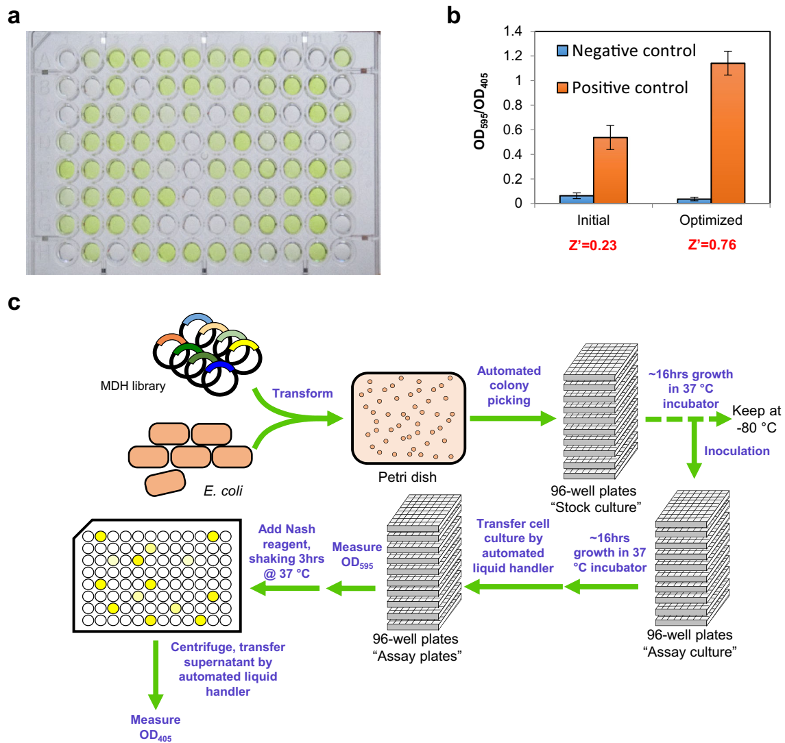
Fig. 5 Development of HTS for Mdh. a Utilizing the colorimetric Nash reaction to measure Mdh activity. The yellow color indicates reaction product diacetylhydrolutidine and can be quantified by OD 405 . b Optimization of HTS process by showing improved Z'-factor. Wild-
