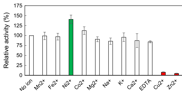
Fig. 2 Effect of ions and chelator to Mdh2. Experiments were performed by incubating enzyme with 1 mM ions (0.1 mM for \text{Cu}^{2+} and \text{Zn}^{2+} ) or EDTA for 3 min, then using 800 mM methanol and 3 mM \text{NAD}^+ as substrates at 30 °C and pH 9.5. The highlighted green color indicates significant activity increase and red color indicates significant activity decrease. The data shown were from triplicate experiments
