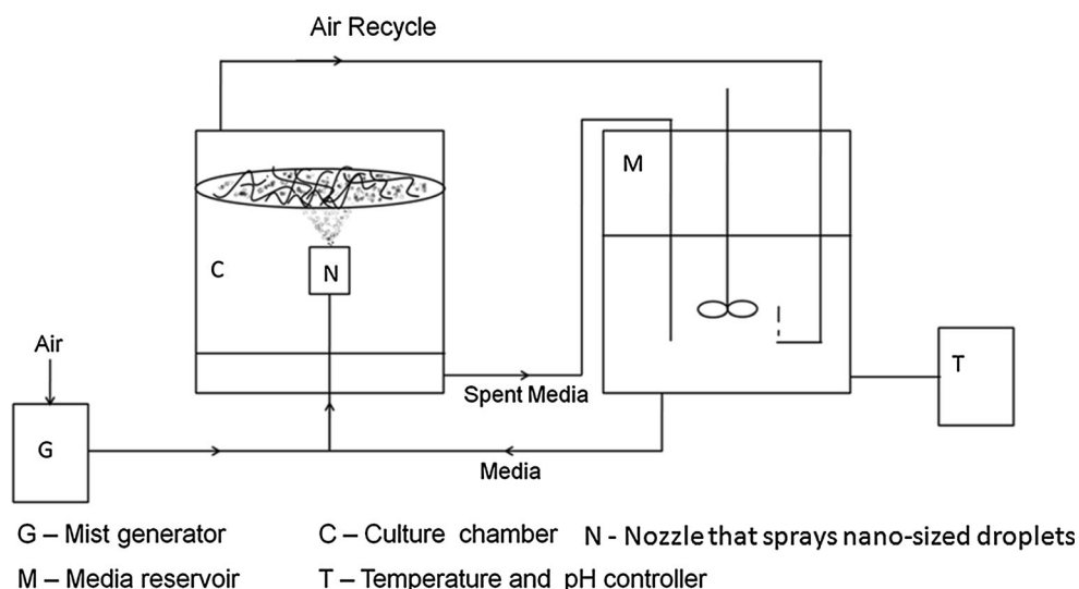
Fig. 2 Schematic diagram of nutrient mist reactor
