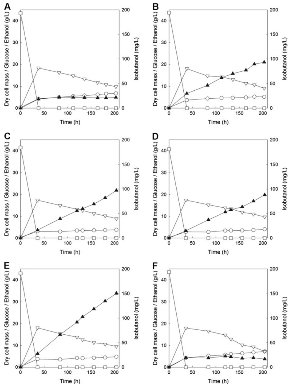
Fig. 4 Profiles of micro-aerobic batch fermentations of recombinant S. cerevisiae D-56 (a), D-K (b), D-I3K (c), D-I53K (d), D-I253K (e) and D-I253 (f). Dry cell mass (open circle), glucose (open square), ethanol (inverted triangle) and isobutanol (closed triangle). Measurements of cell, glucose, ethanol, and isobutanol concentrations were done by three independent experiments of the six strains. Symbols in the figures show the representative values of batch fermentations
