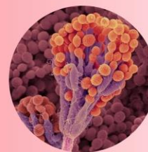
Penicillium chrysogenum
