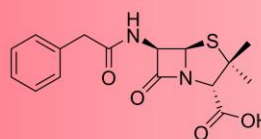
Penicillin (antibiotic)
