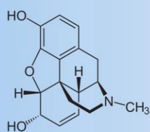
Morphine (analgesic)
