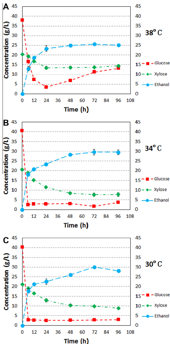
Fig. 2. The effects of temperature on the inhibitor tolerance of S. cerevisiae SyBE005. A: SSsCF at 38 °C; B: SSsCF at 34 °C; C: SSsCF at 30 °C. The fermentation conditions include: inoculation size 2.5 g/L, 12 h pre-hydrolysis, pH 5.5 and 15% (w/w) DM (dry matter) loading.
