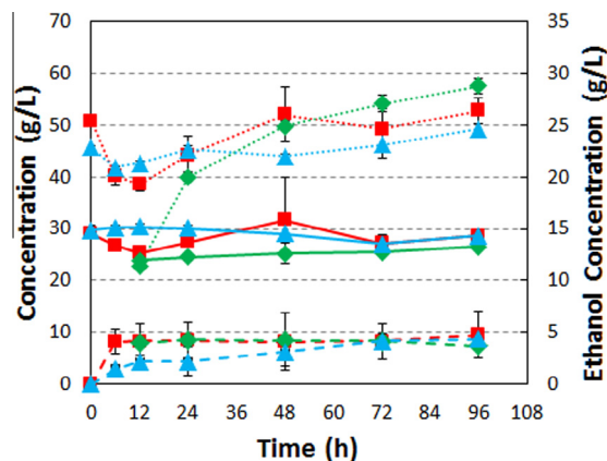
Fig. 3. SSsCF performance of S. cerevisiae SyBE005 with different strategies at 20% (w/w) DM loading. PF: SSsCF with pre-fermentation. YF: SSsCF with yeast feeding. G: glucose. X: xylose. E: ethanol. The fermentation conditions include: inoculation size 2.5 g/L, 12 h pre-hydrolysis, pH 5.5. SSsCF with pre-fermentation was conducted without pre-hydrolysis.
