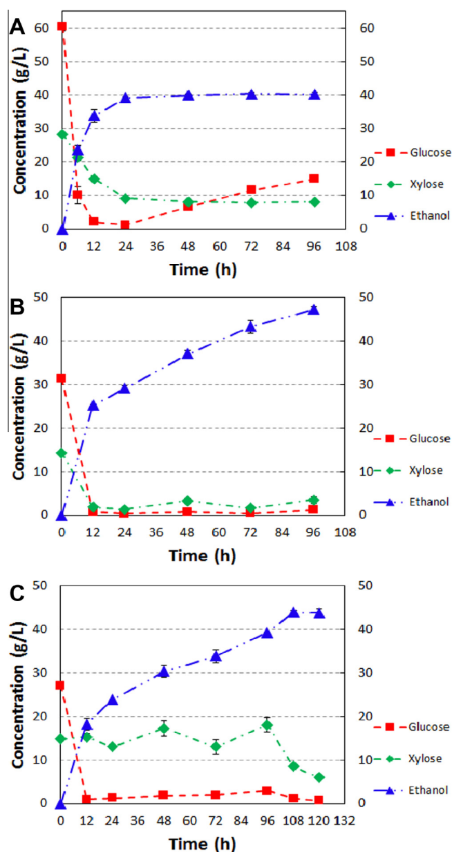
Fig. 6. The effect of high yeast inoculum size on SSf at 25% (w/w) DM loading. A: fermentation performance of batch SSf with 7.5 g/L yeast. B: fermentation performance of fed-batch SSf with 7.5 g/L yeast at 0 h. C: fermentation performance of fed-batch SSf with 2.5 g/L yeast at 0 h and 5.0 g/L yeast at 96 h.
