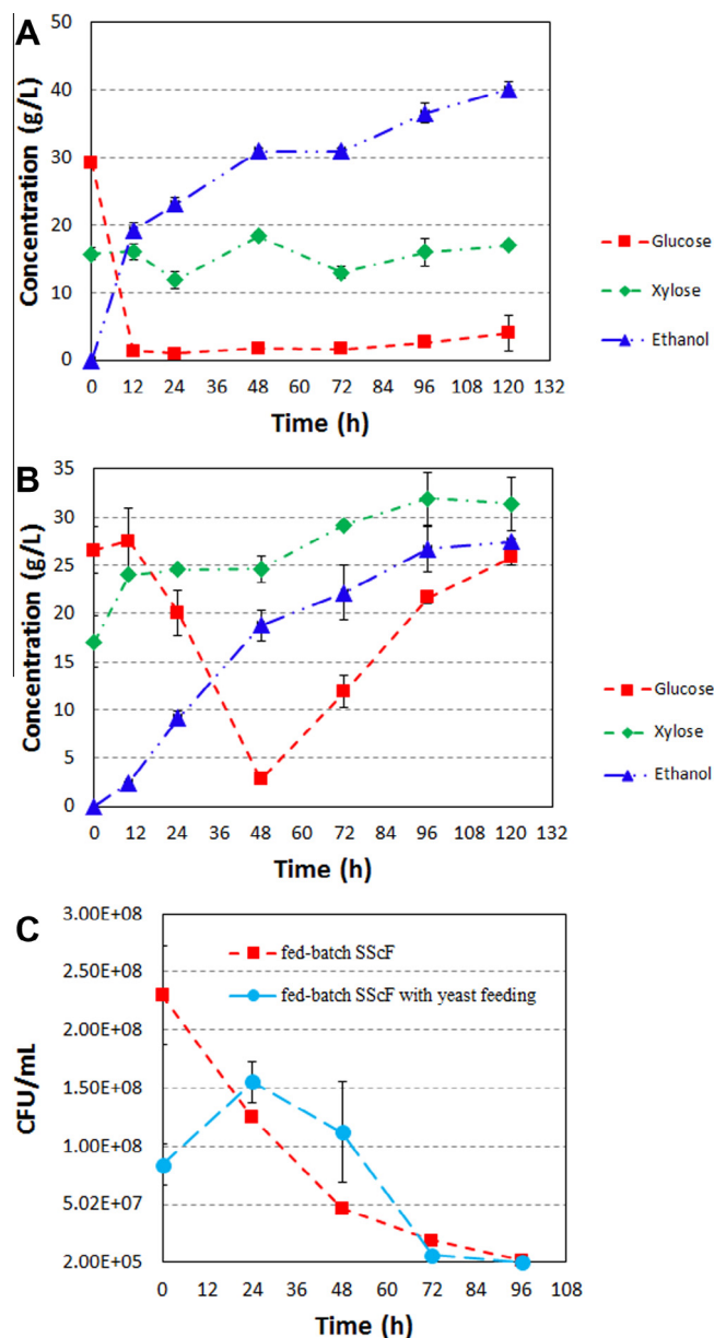
Fig. 5. The effect of fed batch of biomass and yeast feeding of SSf at 25% (w/w) DM loading. A: fermentation performance of SSf with fed batch of biomass. B: fermentation performance of fed-batch SSf with yeast feeding. C: cell viability during SSf with fed batch of biomass and yeast feeding.
