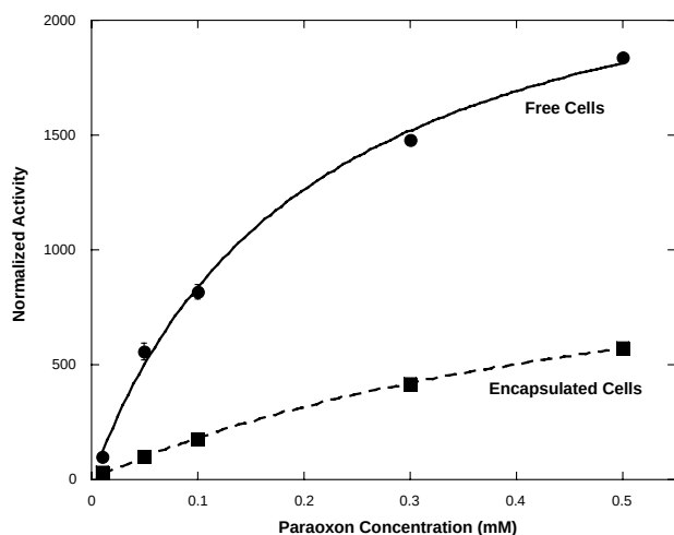
Fig. 2. Michaelis–Menten kinetics of paraoxon hydrolysis using cell-surface-expressed OPH. Comparison of free and encapsulated (sodium silicate process) recombinant Moraxella spp. cells. Free cells: K_m , 0.16 mM; V_{max} , 2221 AU/min OD 600 ; encapsulated cells: K_m , 0.58 mM; V_{max} , 1232 AU/min OD 600 . Standard error for each data point is as shown.
