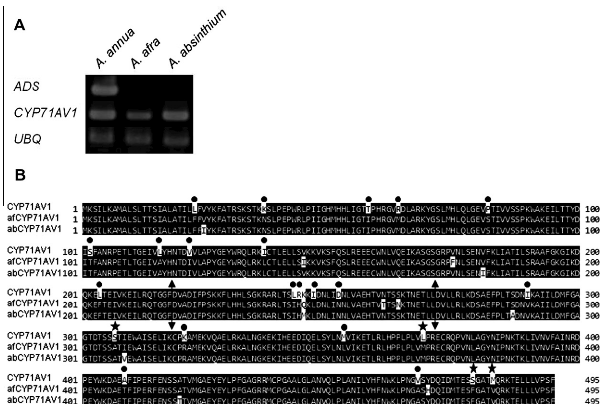
Fig. 1. Isolated putative CYP71AV1 orthologs from A. afra and A. absinthium . (A) RT-PCR analysis of amorpho-4,11-diene synthase ( ADS ) and CYP71AV1 mRNA levels in leaves. Ubiquitin ( UBQ ) was included as an internal control. (B) Alignment of deduced amino acid sequences of CYP71AV1 and putative CYP71AV1 orthologs (GENETYX Version 8; GENETYX Corp., Tokyo, Japan). Identical residues are indicated by dark shading. The large double arrows indicate the three regions of chimeric proteins. Circled marks and stars denote the conserved regions in afCYP71AV1 and abCYP71AV1 that differ in CYP71AV1. Stars show the positions of site-directed mutations.
