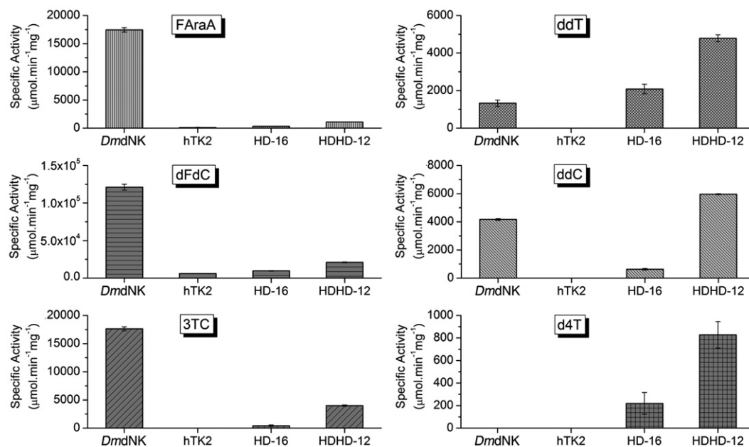
Figure 3. Specific activities of DmdNK , hTK2, HD-16 and HDHD-12 for phosphorylation of the following nucleoside analogs: FdAraA (2-fluoro-9 \beta -D-arabinofuranosyladenine), dFdC (2',2'-difluorodeoxycytidine), 3TC (2'-deoxy-3'-thiacytidine), ddT (2',3'-dideoxythymidine), ddC (2',3'-dideoxycytidine) and d4T (2',3'-didehydro-3'-deoxythymidine). No catalytic activity towards the NAs GCV (ganciclovir), ACV (acyclovir) and ddI (2',3'-dideoxyinosine) was detected.
