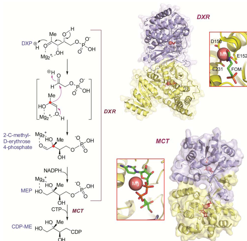
Figure 4. Mechanism of reaction, structure and key features of DXR and MCT. The top structure shows the DXR dimer with the subunits colored either blue or yellow in association with the inhibitor fosmidomycin (FOM in red) based on its reported structure (PDB 1ONP). 61c Inset indicates FOM and the critical residues D150, E152, and E231 (colored by heteroatoms) that coordinate the divalent ion ( \text{Mn}^{2+} ) within the active site of DXR. The MCT dimer structure with the subunits colored either blue or yellow in complex with its product CDP-ME (red) is based on its reported structure (PDB 3Q80). Inset shows the orientation of CDP-ME in relation to the \text{Mg}^{2+} ion within the active site of MCT. The mechanism of reaction of DXR is adapted from with permission from ref 58. Copyright 2008 American Chemical Society.
