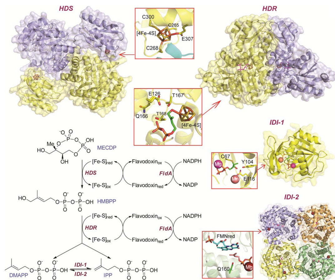
Figure 6. Mechanism of reaction, structure and key features of HDS, HDR, IDI-1, and IDI-2. The reductive reactions carried out by HDS and HDR indicate the coupling to electrons obtained via flavodoxin and flavodoxin reductase (FldA) from NADPH. Top left, the HDS dimer structure with the subunits colored either blue or yellow based on its reported structure (PDB 3NOY). 87a Inset indicates the critical C265, C268, C300, and E307 residues of HDS that coordinate the iron sulfur cluster ([4Fe-4S]) (colored by heteroatoms). Top right, the HDR dimer structure with the subunits colored either blue or yellow based on its reported structure (PDB 3KE8) in complex with HMBPP substrate (red). 88c The inset indicates the iron sulfur cluster ([4Fe-4S]) and the critical Q166, T167, T168, and E126 residues (colored by heteroatoms) of HDR. Middle right, the structure of E. coli IDI-1 monomer (PDB 1NFZ) following treatment with the irreversible inhibitor 3,4-epoxy-3-methyl-1-butyl diphosphate. 109a Inset indicates the orientation of 4-hydroxy-3-methyl butyl diphosphate linked to the sulfur group of C67 and in relation to the Mg^{2+} and Mn^{2+} divalent ions and the critical residues E116, Y104 (colored by heteroatoms) of IDI-1. Bottom right, the structure of IDI-2 tetramer with each subunit colored in either blue, orange, teal, or yellow based on its reported structure (PDB 3B05). 116a Inset indicates the critical residue Q160 and the reduced FMN (FMNred) cofactor of IDI-2. Bottom left, diagram indicates the mechanism of the HDS, HDR, and IDI-1 and IDI-2 catalyzed reactions adapted from reference with permission from ref 283. Copyright 2007 American Society for Biochemistry and Molecular Biology.
