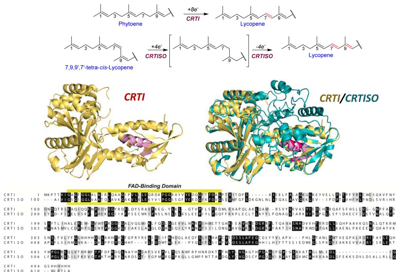
Figure 10. Enzymatic reaction, structure, and key features of CRTI and CRTISO. The desaturation reaction catalyzed by CRTI is shown in comparison with the saturation-isomerization-desaturation reaction catalyzed by CRTISO. Bottom left, the structure of CRTI is based on its reported structure (PDB 4DGK) indicating the FAD binding \beta - \alpha fold (pink). 152c Bottom right, a prediction of the structure of tomato CRTISO using I-TASSER 144 is colored in teal and is superimposed on the CRTI structure colored in gold. The FAD binding domain of CRTISO (purple) and that of CRTI (pink) are indicated. Below, the alignment of the sequence of hexahistidine tagged-CRTI (as used to generate the PDB 4DGK structure) and tomato CRTISO with identical residues in white letters on black background and conserved substitutions in black on gray background. The extended FAD binding domain shared by CRTI, CRTISO, and protoporphyrinogen oxidoreductases and monoamine oxidase is highlighted in yellow. The diagrams depicting reactions of CRTI and CRTISO is adapted and reprinted with permission from reference from ref 197b. Copyright 2005 Elsevier.
