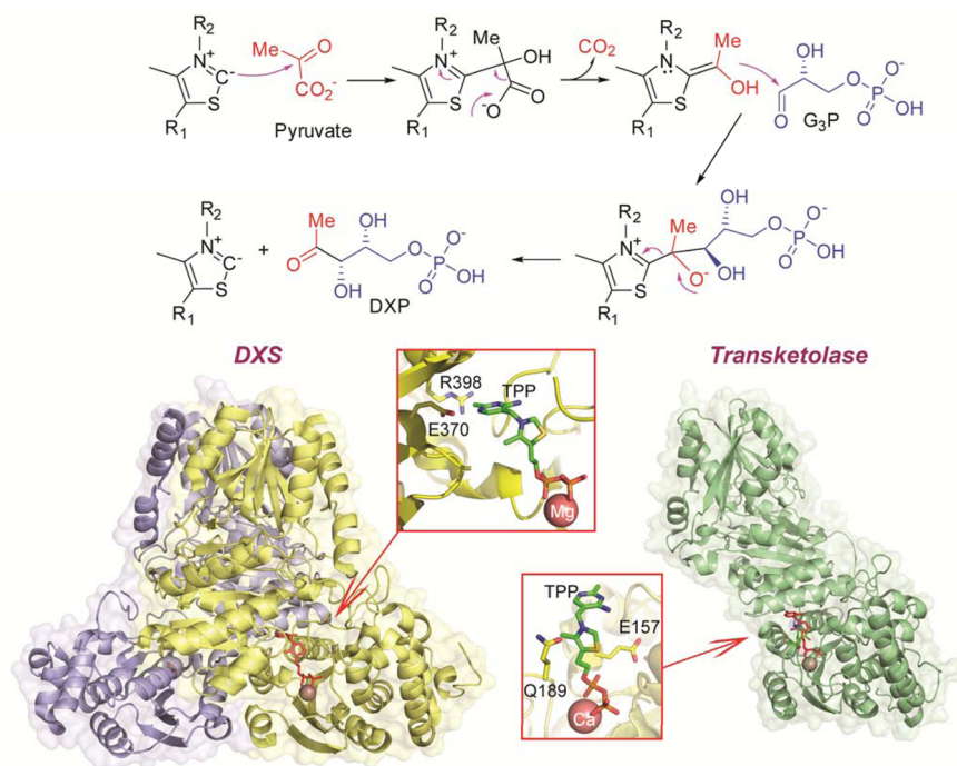
Figure 3. Mechanism of reaction, structure, and key features of DXS in comparison with transketolase. At left, the structure of the DXS dimer in complex with TPP (red) based on its reported structure (PDB 2O1S) with the subunits colored either blue or yellow. 46 Inset shows the orientation of TPP and the critical E370 and R398 residues of DXS colored by heteroatoms. Right structure shows a monomer of the related transketolase structure (PDB 3MOS) (green) in combination with TPP (red). 282 Inset shows the important transketolase E157 and Q189 residues involved in binding TPP colored by heteroatoms. The mechanism of reaction of DXS is adapted and reprinted with permission from ref 44. Copyright 2003 American Chemical Society.
