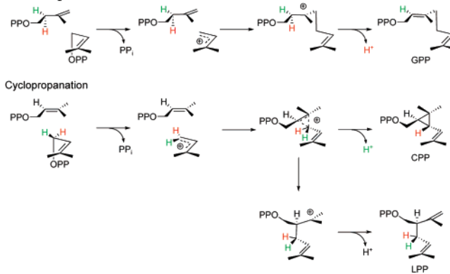
Scheme 2 Chain Elongation
