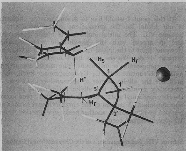
Figure 3. Cyclobutyl cation.
