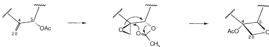
Fig. 3 A possible mechanism for the construction of the oxetane ring of taxol from the 4(20)-ene-5 \alpha -acetate functional grouping. Epoxidation of the 4(20)-double bond, followed by intramolecular acetate migration and oxirane ring opening, could furnish the oxetane moiety.
