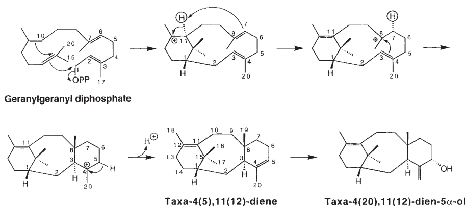
Fig. 2 Stereochemical mechanism for cyclization of geranylgeranyl diphosphate to taxa-4(5),11(12)-diene involving 1S-verticillene as a transient intermediate. A single enzyme base (not illustrated) is responsible for removal of the 11 \alpha -hydrogen and reprotonation at C-7. Hydroxylation at C-5 of taxa-4(5),11(12)-diene, with migration of the double bond, to afford taxa-4(20),11(12)-dien-5 \alpha -ol is also shown.
