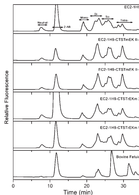
Fig. 8. Anion-exchange HPLC analysis of 2-AB-labeled N-linked glycans from rhEPO. N-Linked glycans from purified rhEPO were derivatized with 2-AB and then separated on anion-exchange column (DEAE-5PW; Tosoh) according to the number of sialic acid residues. Peaks of sialylation profiles were identified by comparison to standard 2-AB-bovine fetuin N-linked glycan library (Glyko®). 2-AB peak indicates the non-bound 2-AB reagent.
