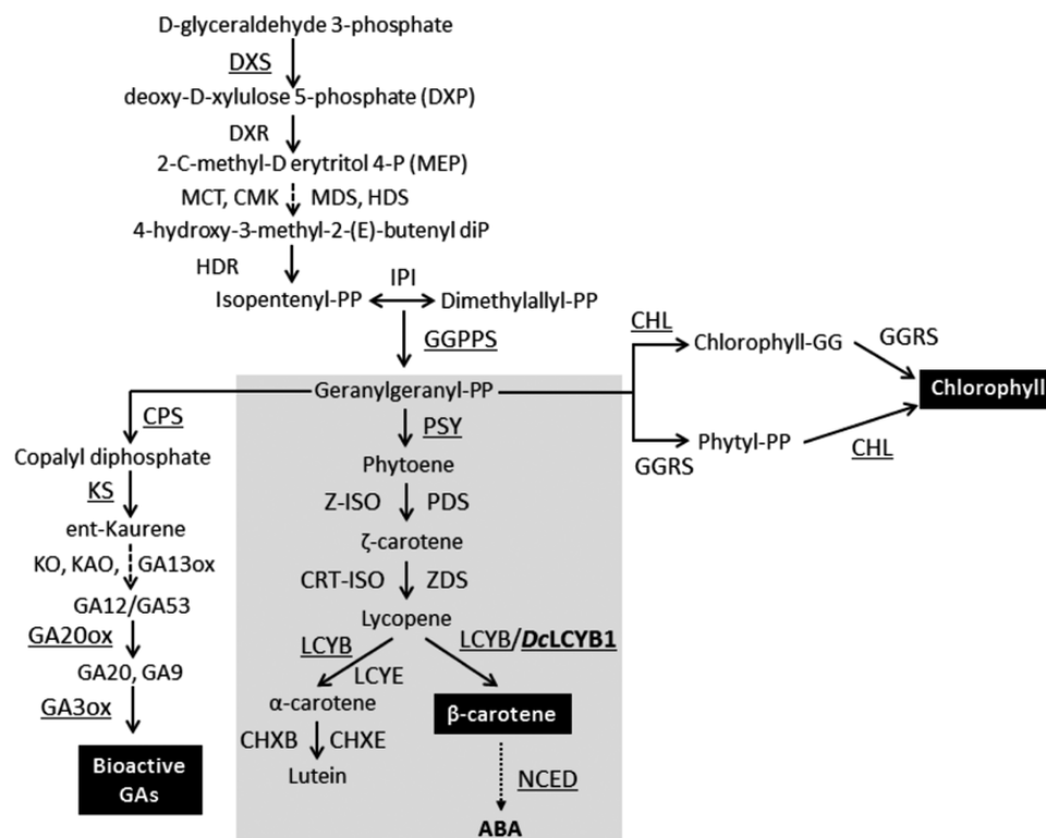
Fig. 1. Carotenoid and directly-related biosynthesis pathways. Enzymatic conversions are shown by arrows with the enzymes involved in each reaction. The carotenoid pathway is in the center of the figure enclosed in grey, flanked by the chlorophyll and gibberellin (GA) pathways. Genes analyzed in this work are underlined. The non-mevalonate pathway (MEP) takes place in plastids to produce geranylgeranyl pyrophosphate (GGPP) that is required for carotenoid, chlorophyll and gibberellin synthesis, among others. DXS, deoxyxylulose synthase; DXR, 1-deoxyxylulose 5-phosphate reductoisomerase; CMS, 2C-methyl-D-erythritol 4-phosphate cytidyltransferase, CMK, 4-(cytidine 5-diphospho)-2-C-methyl-D-erythritol kinase, MCS, 2C-methyl-D-erythritol 2,4-cyclodiphosphate synthase, HDS, 4-hydroxy-3-methylbut-2-enyl diphosphate synthase; HDR, 4-hydroxy-3-methylbut-2-enyl diphosphate reductase; IPI, isopentenyl diphosphate isomerase; GGPPS, geranylgeranyl pyrophosphate synthase; PSY, phytoene synthase; PDS, phytoene desaturase; Z-ISO, z-carotene isomerase; ZDS, Z-carotene desaturase; CRT-ISO, carotenoid isomerase; LCYB, lycopene \beta -cyclase; LCYE, lycopene \epsilon -cyclase; CHXB, \beta -carotene hydroxylase; CHXE, \epsilon -carotene hydroxylase; GGRS, geranylgeranyl reductase; CHL, chlorophyll synthase; CPS, copalyl diphosphate synthase; KS, ent-kaurene synthase; KO, ent-kaurene oxidase; KAO, ent-kaurenoic acid oxidase; GA20ox, GA 20-oxidase; GA3ox, GA 3-oxidase; NCED, 9-cis-epoxycarotenoid dioxygenase. The LCYB1 enzyme from Daucus carota which was overexpressed in this work is boldfaced in the respective reaction of the pathway. The enzymes for which the expression of their corresponding coding sequences was quantitatively analyzed by qRT-PCR are underlined. Dashed lines represent multiple reaction steps.
