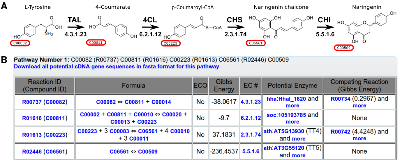
Figure 5. A heterologous biosynthesis pathway to produce naringenin from L-tyrosine in an E. coli host. (A) The structure of an experimentally derived biosynthesis pathway (29). The EC number for each reaction is indicated below the arrow. The KEGG compound ID of each metabolite is framed in red. The abbreviations are: tyrosine ammonia lyase (TAL); 4-coumarate:CoA ligase (4CL); chalcone synthase (CHS) and chalcone isomerase (CHI). (B) The information of the top-ranked biosynthesis pathway in MRE.
