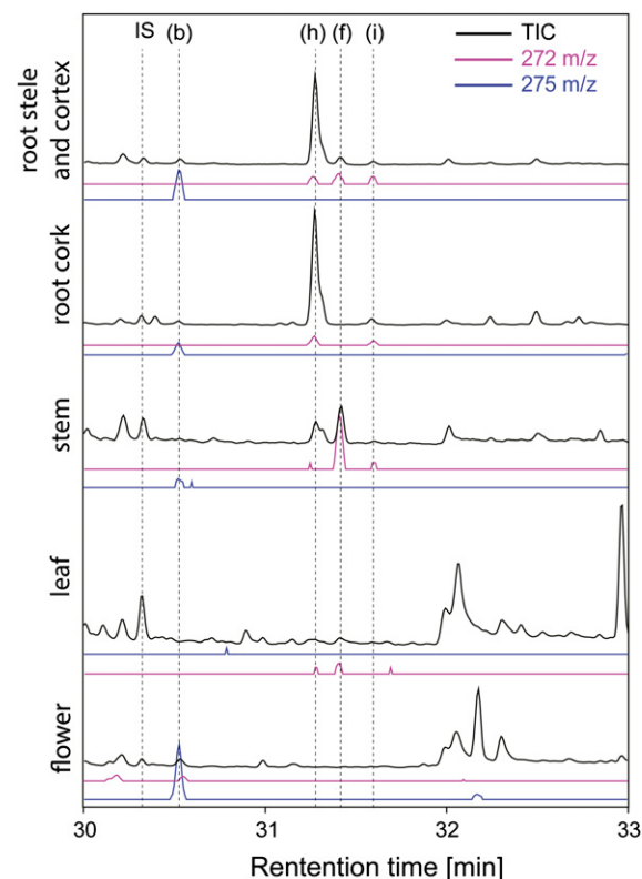
Figure 4. GC-MS analysis of hexane extracts from C. forskohlii tissues. The letter “b” indicates (13R) manoyl oxide, “h” indicates dehydroabietadiene, “f” indicates multiradiene, and “i” indicates abietadiene. IS, Internal standard (1 mg L -1 1-eicosene).
