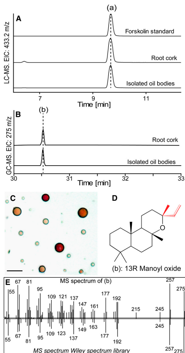
Figure 3. Detection of forskolin (a) and (13R) manoyl oxide (b) in C. forskohlii root cork and isolated oil bodies. A, LC-MS EIC of m/z 433.2197 [forskolin + Na] ^+ in isolated oil bodies and in root cork tissue from C. forskohlii . B, GC-MS EIC of m/z 275 corresponding to manoyl oxide in isolated oil bodies and in root cork tissue from C. forskohlii . C, Bright-field microscope image of isolated C. forskohlii oil bodies. Bar = 5 \mu m. D, Molecular structure of (13R) manoyl oxide. E, Mass spectrum obtained from manoyl oxide identified in root cork tissue (top) and reference spectrum (bottom) from Wiley mass spectrum database.
