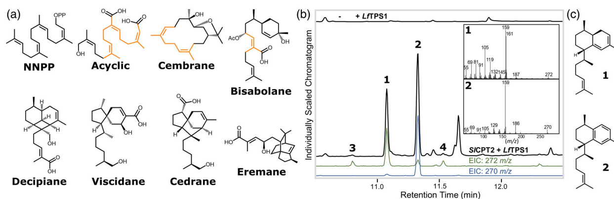
Figure 3. Dihydroserulatene production by Lf TPS1. (a) Structure of NNPP and representative non-serrulatane diterpenoids from Eremophila with labeled backbone structure types. Isoprenyl subunits found in acyclic, cembrane, and bisabolane type diterpenoids, which can be used to infer the stereochemistry of their prenyl diphosphate precursor, are highlighted in orange. (b) Transient expression of Lf TPS1 in N. benthamiana with SICPT2 (a plastidial NNPP synthase), and mass spectra of major products. Each assay has Cf DXS co-expressed in addition to those listed. (c) Structures of dihydroserulatene (1) and serrulatene (2).
