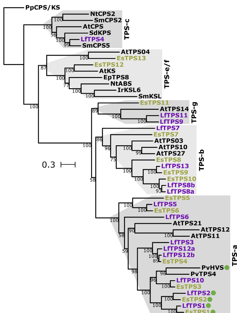
Figure 2. Maximum likelihood phylogenetic tree of TPS candidates. Candidate terpene synthases from L. frutescens and E. serrulata are shown in purple and yellow, respectively, with reference TPSs in black. Putative transit peptides, predicted by N-terminal extensions, are denoted within the TPS-a subfamily.
