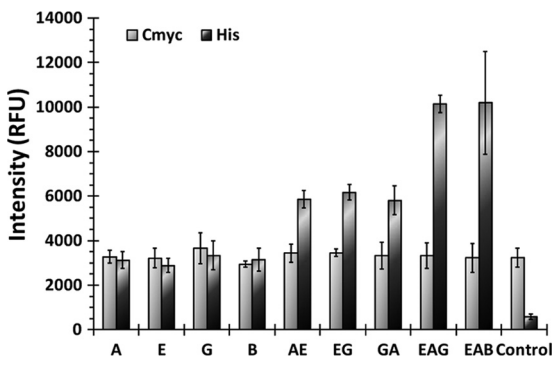
FIG. 3. Fluorescence intensity of cells either displaying scaffoldin Scaf-ctf or with different combinations of dockerin-tagged cellulases (At [A], Ec [E], and Gf [G]) docked on the displayed Scaf-ctf. Cells were probed with either anti-c-Myc or anti-c-His 6 serum and fluorescently stained with goat anti-mouse IgG conjugated with Alexa Fluor 488. Whole-cell fluorescence was determined with a fluorescence microplate reader. Cells displaying only Scaf-ctf were used as controls. RFU, relative fluorescence units.
