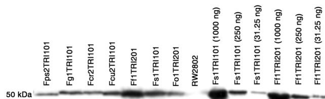
FIG. 2. Western blot of TRI101/TRI201 enzymes from F. pseudograminearum (Fps2TRI101), F. graminearum (Fg1TRI101), F. crookwellense (Fcr2TRI101), F. culmorum (Fcu2TRI101), F. fujikuroi (Ff1TRI201), F. sporotrichioides (Fs1TRI101), and F. oxysporum (Fo1TRI201) (1 and 2 indicate that the strain is from the Schmale or Leslie collection, respectively). Protein extracts from yeast cultures were collected following 24 h of expression. Untransformed yeast strain RW2802 represents the negative control. Ten microliters of each protein extract was loaded onto a 12% acrylamide-SDS-PAGE gel and run at 150 V for 1 h. Precision plus protein dual color standard was used to determine protein size. Ten microliters of TRI101 from F. sporotrichioides and TRI201 from F. fujikuroi , both purified from E. coli , were loaded as positive controls at known amounts of 1,000 ng, 250 ng, and 31.25 ng. The Western blot was probed with rabbit anti-FsTRI101 primary antibody and detected with alkaline phosphatase-conjugated anti-rabbit antibody.
