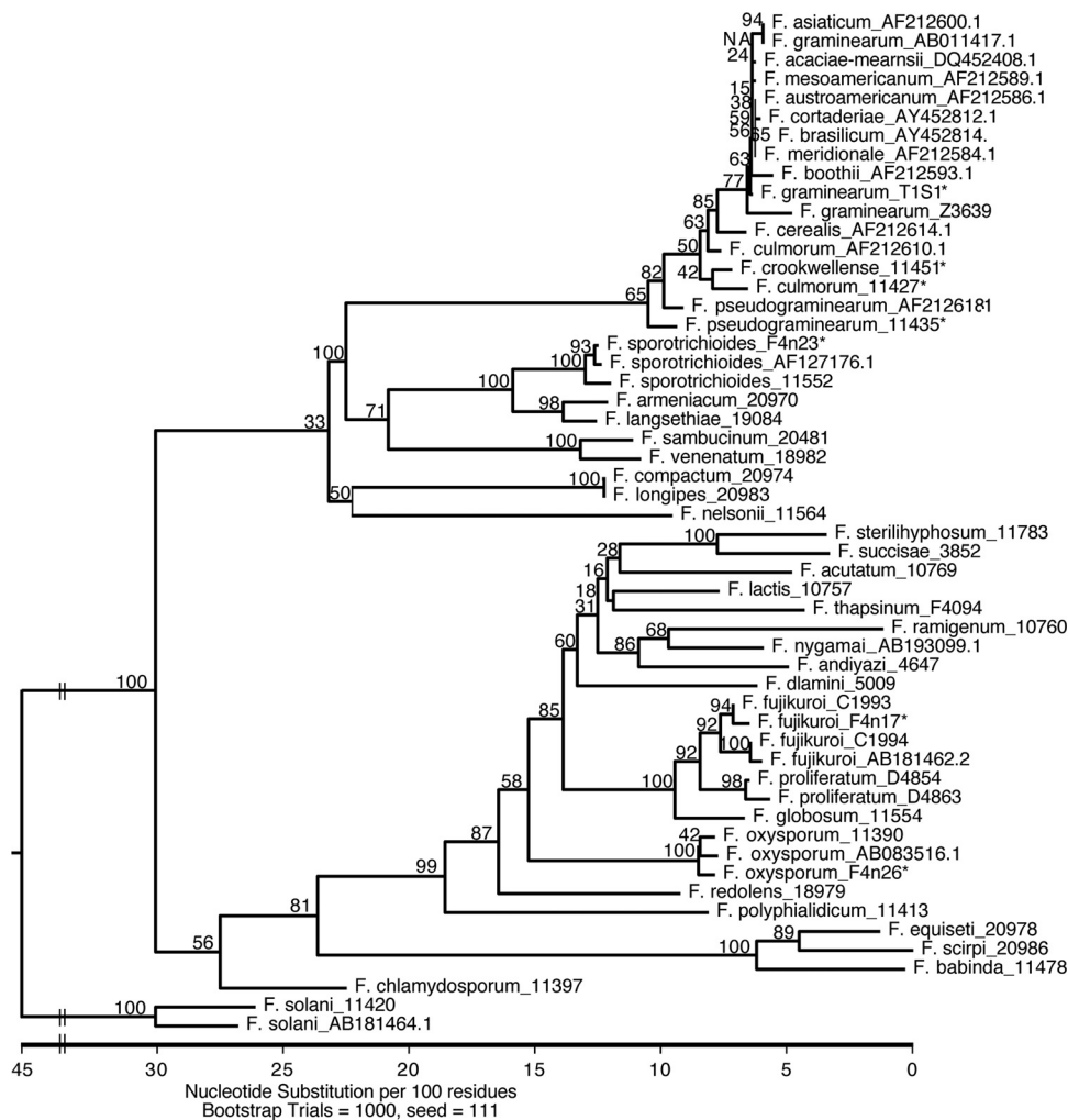
FIG. 1. Phylogenetic tree based on a total of 688 bp of sequence internal to the 3' end of TRI101/TRI201 . Sequences included in the tree are from a total of 54 strains of Fusarium : 33 strains from the Leslie collection (see Table S2 in the supplemental material), four strains from the Schmale collection, and 17 strains from GenBank (see Table S1 in the supplemental material). Strain numbers or GenBank accession numbers follow the underscores. *, species whose full-length TRI101/TRI201 gene products were analyzed in this study for their ability to detoxify DON. Numbers at branch points represent bootstrap values.
