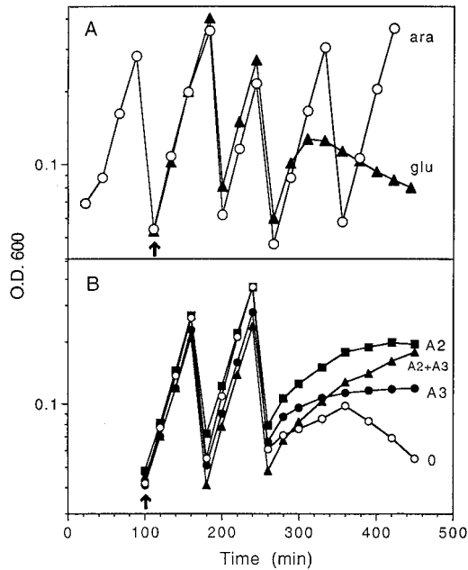
FIG. 2. Growth of MGΔ Ly after depletion of LytB . Cultures grown in LB medium containing 0.2% arabinose and 50 μg of ampicillin per ml were diluted and grown in the same medium for 3.5 generations. At the times indicated by the arrows cultures were diluted into medium with arabinose or glucose (0.2%). Cultures were maintained in the exponential phase at all times. Large decreases in optical density at 600 nm (O.D. 600) indicate times of dilution. (A) Growth with arabinose or glucose; (B) cultures contain glucose and each of the alcohols indicated at a concentration of 10 mM.
