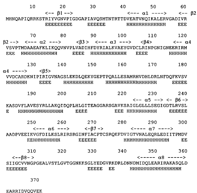
FIG. 5. Predicted secondary and tertiary structures for GcpE. H and E beneath the protein sequence indicate that the corresponding residues are predicted by PHD (21) to form parts of an \alpha -helix and an extended structure ( \beta -sheet), respectively. Information above the sequence indicates the predicted positions and extents of the backbone \alpha - and \beta -units of the TIM barrel tertiary structure, inferred from a comparison of the sequences of homologues of GcpE and of the PDB structure 1THF.
