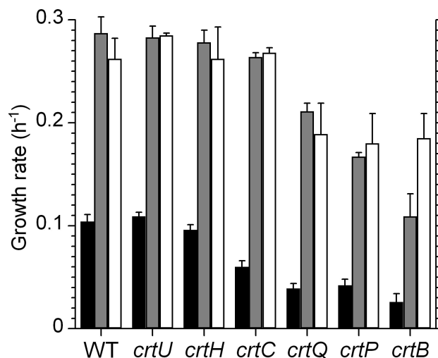
FIG. 7. Growth rates of the wild-type and mutant strains of C. tepidum at various light intensities. The light intensities used were 10 (black bars), 76 (shaded bars), and 588 (white bars) \mu mol of photons m -2 s -1 . The data are the means \pm standard deviations (error bars) from at least four separate experiments. WT, wild type.
