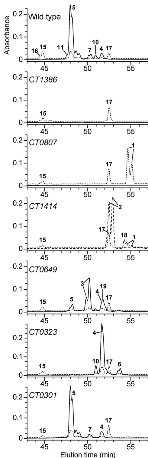
FIG. 4. HPLC chromatograms of cell extracts of the wild-type and mutant strains of C. tepidum with detection wavelengths of 270 nm (---), 400 nm (— — —), and 490 nm (——). The amount of extract injected corresponded to about 10 \mu g of BChl c . Peaks are identified in Table 1. Other peaks are as follows: peak 13, OH- \gamma -carotene glucoside (35.6 min); peak 14, OH-chlorobactene glucoside (30.3 min); peak 15, chlorobiumquinone 7 (44.8 min); peak 16, 1'-hydroxymenaquinone 7 (44.5 min); peak 17, menaquinone 7 (52.5 min); peak 18, 1,2-dihydro- \zeta -carotene (54.2 min); and peak 19, 1,2-dihydrolycopene (51.8 min).
