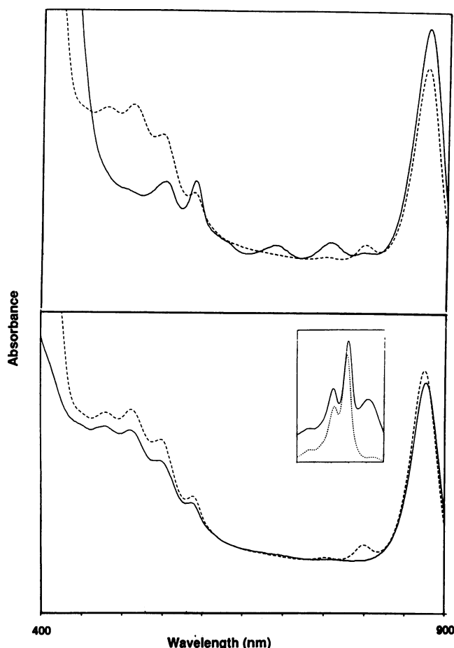
FIG. 4. Spectral analysis of R. centenum mutants. (Top) Spectral analysis of the crtI mutant FY011. ---, absorbance spectrum generated from photosynthetically grown wild-type R. centenum ; —, spectrum obtained from the photosynthetically grown crtI mutant FY011. (Bottom) Spectral analysis of the reaction center-deficient strain FY059. ---, absorbance spectrum obtained from wild-type R. centenum ; —, absorbance spectral analysis of the reaction center-deficient strain FY059. The inset is a spectral analysis of a reaction center preparation, obtained from wild-type cells, that was scanned under reduced (—) and ferricyanide oxidized (---) conditions (preparation of R. centenum reaction centers will be described elsewhere [37a]). The reaction center has a major peak at 800 nm and an oxidizable peak at 850 nm.
