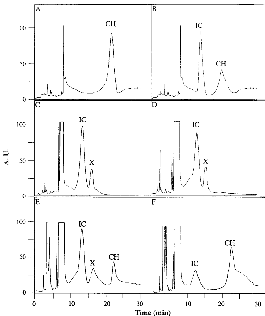
FIG. 5. Determination of the reversibility of the reaction. For the forward reaction, the standard reaction mixture with chorismate was used, and for the reverse reaction, the chorismate in the reaction mixture was replaced by isochorismate. After incubation, the product(s) formed was determined as described in Materials and Methods. (A) Chorismate without enzyme; (B) complete reaction mixture with MenF and chorismate; (C) isochorismate without enzyme; (D) complete reaction mixture with MenF and isochorismate; (E) complete reaction mixture with EntC and isochorismate; (F) complete reaction mixture with EntC and chorismate. CH, chorismate; IC, isochorismate; X, unidentified peak. A. U., arbitrary units.
