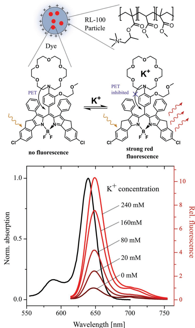
Figure 1. Scheme and spectral properties of K + -sensitive FI3 dye encapsulated in RL100 nanoparticles. Spectra were measured in 20 \times 10^{-3} M Tris-HCl, pH 7.4 with concentration of nanoparticles adjusted to A_{640} = 0.1 .
