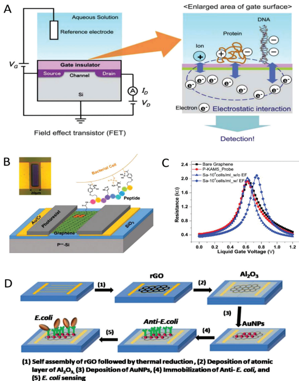
Figure 5. A) Basic design and operation of a FET-based sensor. [81] (Reproduced with permission. [81] Copyright 2013, Royal Society of Chemistry); B) design of the G-FET proposed by Kumar and associates; C) distinct change in variation of resistance with liquid gate voltage with the G-FET and 10^4 SA cells \text{mL}^{-1} . [82] (Reproduced with permission. [82] Copyright 2020, Elsevier); D) schematic showing the design of the FET sensor proposed by Thakur et al. [84] (Reproduced with permission. [84] Copyright 2018, Elsevier).
