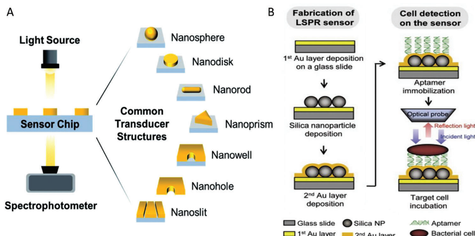
Figure 6. A) Schematic showing a simple plasmonic sensor system with different gold-based surface functionalization. [100] (Reproduced with permission. [100] Copyright 2020, Royal Society of Chemistry); B) schematic showing the design of the platform by Yoo et al. [103] (Reproduced with permission. [103] Copyright 2015, Elsevier).
