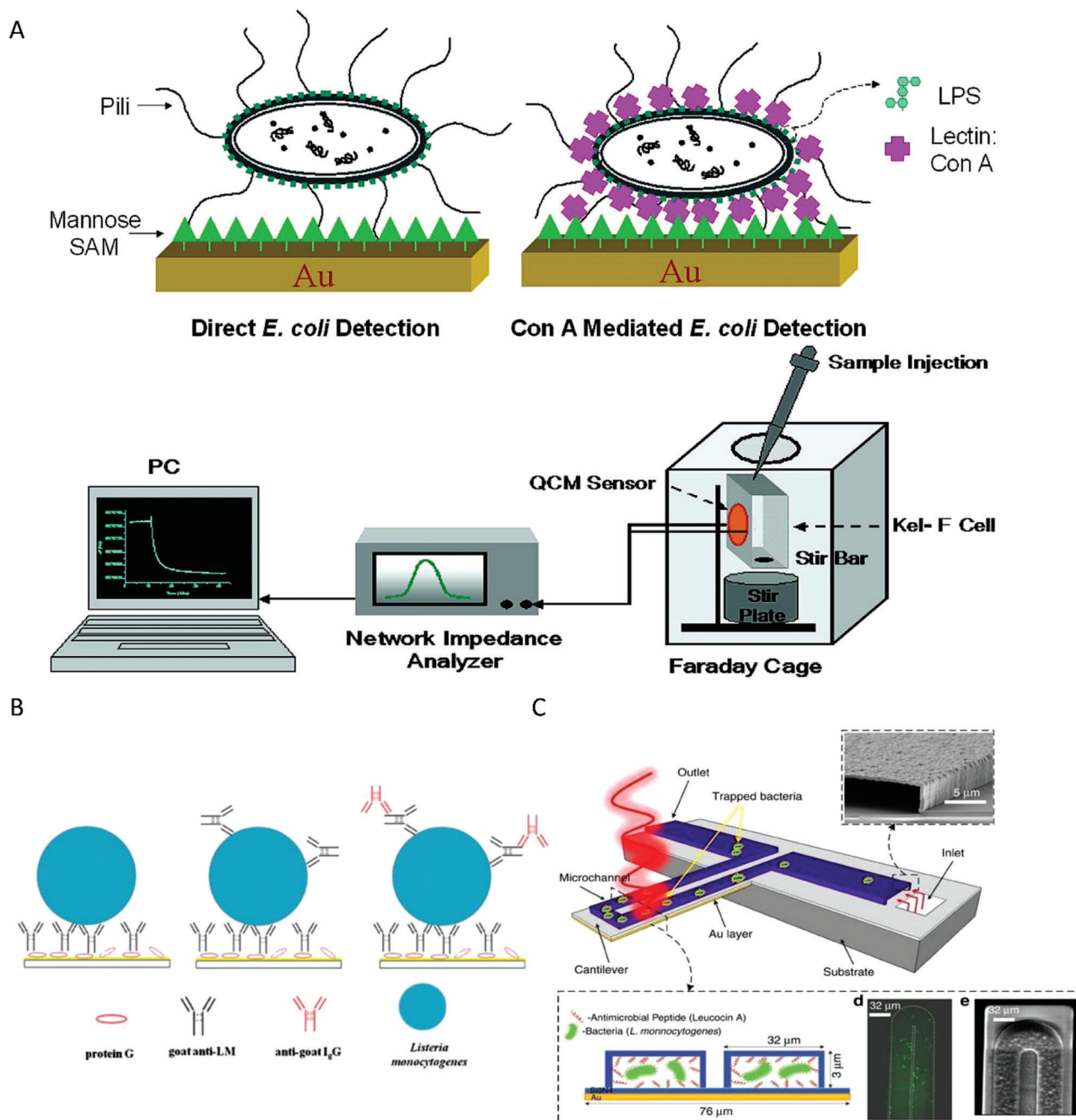
Figure 9. A) Schematic showing the QCM platform designed for E. coli detection. [128] (Reproduced with permission. [128] Copyright 2007, American Chemical Society); B) secondary and tertiary antibody binding design. [129] (Reproduced with permission. [129] Copyright 2013, Elsevier); C) bimetallic cantilever system proposed by Etayash et al. [131] (Reproduced with permission. [131] Copyright 2016, Springer Nature).
