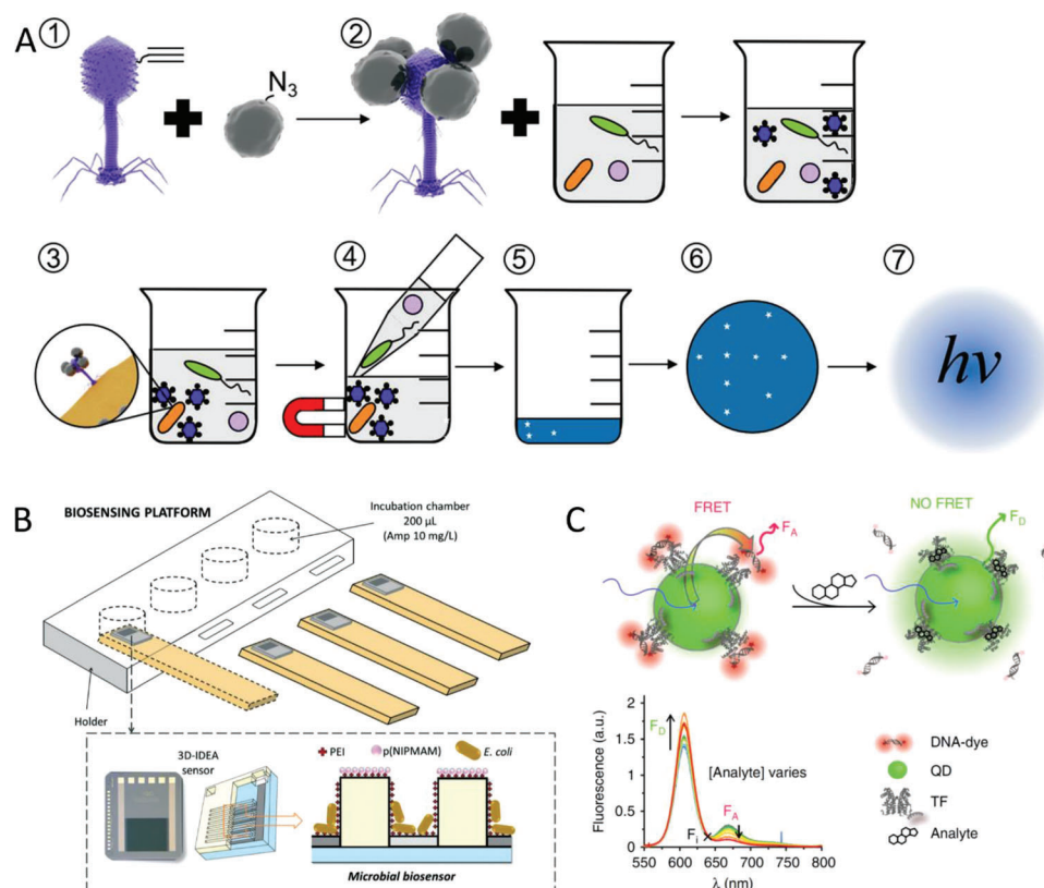
Figure 10. A) Schematic representation of E. coli detection via T4 phage 1) conjugation of alkynylated T4 Nluc CBM phage to the azide coated MNP 2) resulting magnetic phage-based nanobot added to a mixture of bacteria 3) magnetic phage-based nanobot binds to E. coli (orange) 4) beads containing phage and E. coli are collected by magnet 5) infection cycle of T4 phages is completed and Nluc CBM released into the solution 6) sample is filtered on cellulose 7) luminescence arising from T4 phage is measured. [134] (Reproduced with permission. [134] Copyright 2020, American Chemical Society); B) impedance sensing platform by Brosel-Oliu and coworkers. [138] (Reproduced with permission. [138] Copyright 2019, Royal Society of Chemistry); C) FRET process in the detection of progesterone. [139] (Reproduced with permission. [139] Copyright 2020, Springer Nature).
