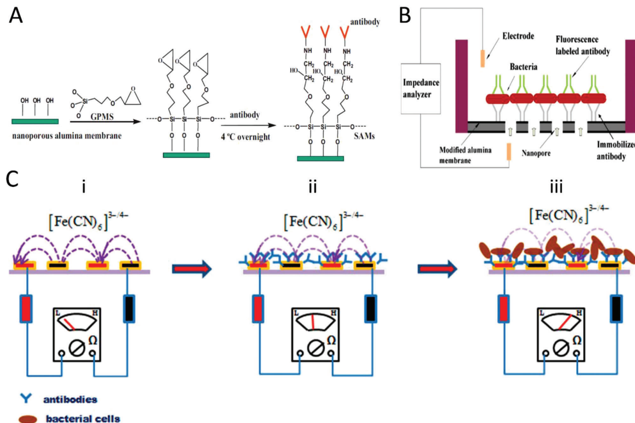
Figure 3. A) Schematic showing the functionalization process of the alumina nanoporous membrane; B) impedimetric biosensor system designed for E. Coli and S. Aureus detection. [43] (Reproduced with permission. [43] Copyright 2011, Elsevier); C) Design of immunosensor i) bare IDAM ii) IDAM functionalized with antibodies iii) bacterial cells captured on IDAM by antibodies (Reproduced with permission. [45] Copyright 2017, MDPI).
