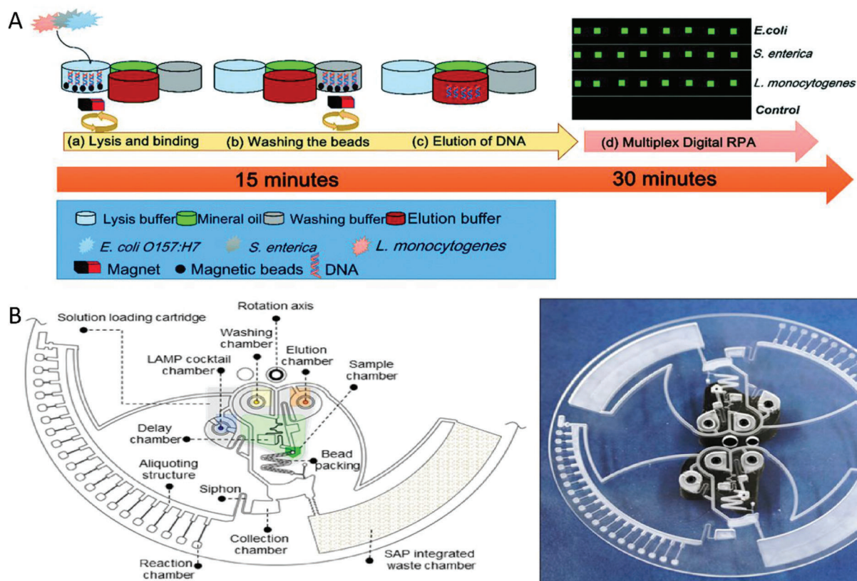
Figure 13. A) Experimental workflow of the sample-in-multiplex-digital-answer-out design by Yin et al. [190] (Reproduced with permission. [190] Copyright 2020, Royal Society of Chemistry); B) schematic illustration of the integrated centrifugal disc and a digital image of the disc. [196] (Reproduced with permission. [196] Copyright 2019, Elsevier).
