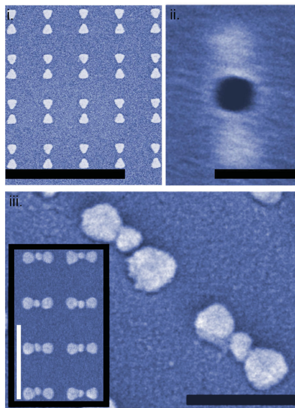
Figure 2. SEM images detailing sensor construction (i) an incomplete bowtie array, (ii) an individual dimer with a 40 nm polymer window aligned to its gap, (iii) coupled devices completed with the inclusion of a DNA-nanoparticle. The scale bars represent 1 \mu\text{m} , 100 nm and 200 nm for SEM images i, ii and iii respectively. The scale bar for (iii)'s inset image is 500 nm. See Experimental Section for full fabrication details.
