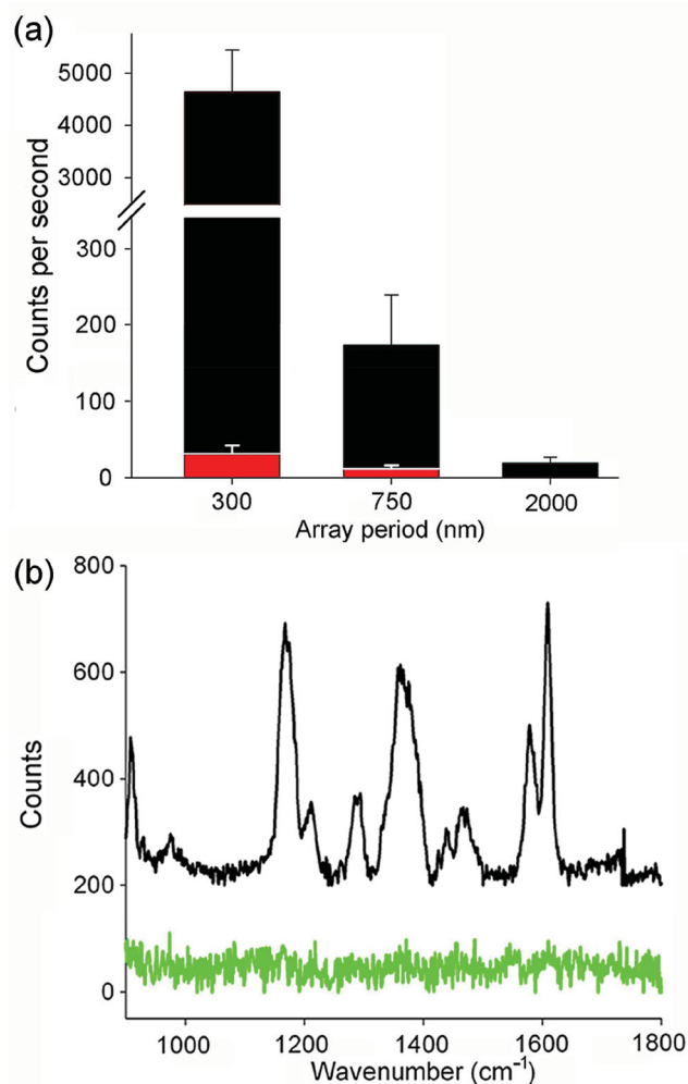
Figure 6. Detecting single nanoparticle binding events. (a) Comparison of SERS intensity, with standard deviation, from the 1605\text{ cm}^{-1} band of malachite green, for different densities of isolated nanoparticles (red bars) and nanoparticles situated in a completed circuit (black bars). 8 measurements were taken for each data point. Acquisition times were 5 seconds for the 300 nm period array and 20 seconds for the 750 and 2000 nm period arrays. Data is presented in counts per second for simplicity of viewing. (b) SERS spectra of a single isolated nanoparticle (green) and a single nanoparticle bound within a plasmonic bowtie via DNA hybridization. The acquisition time was 20 seconds in each case.
