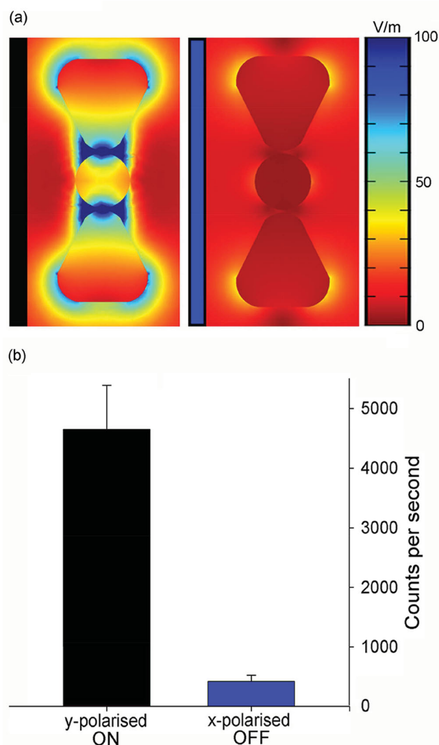
Figure 5. Polarization dependent Raman outputs. (a) FEM simulations of the device excited with the input polarized along the y-axis (left) and the x-axis (right). The side-bar for each simulation represents the normalized electric-field enhancement factor given an incident field value of 1 V/m. (b) Comparison of average SERS intensity, with standard deviation, for a 300 nm period bowtie at these two input conditions. 8 measurements were taken for each input.
