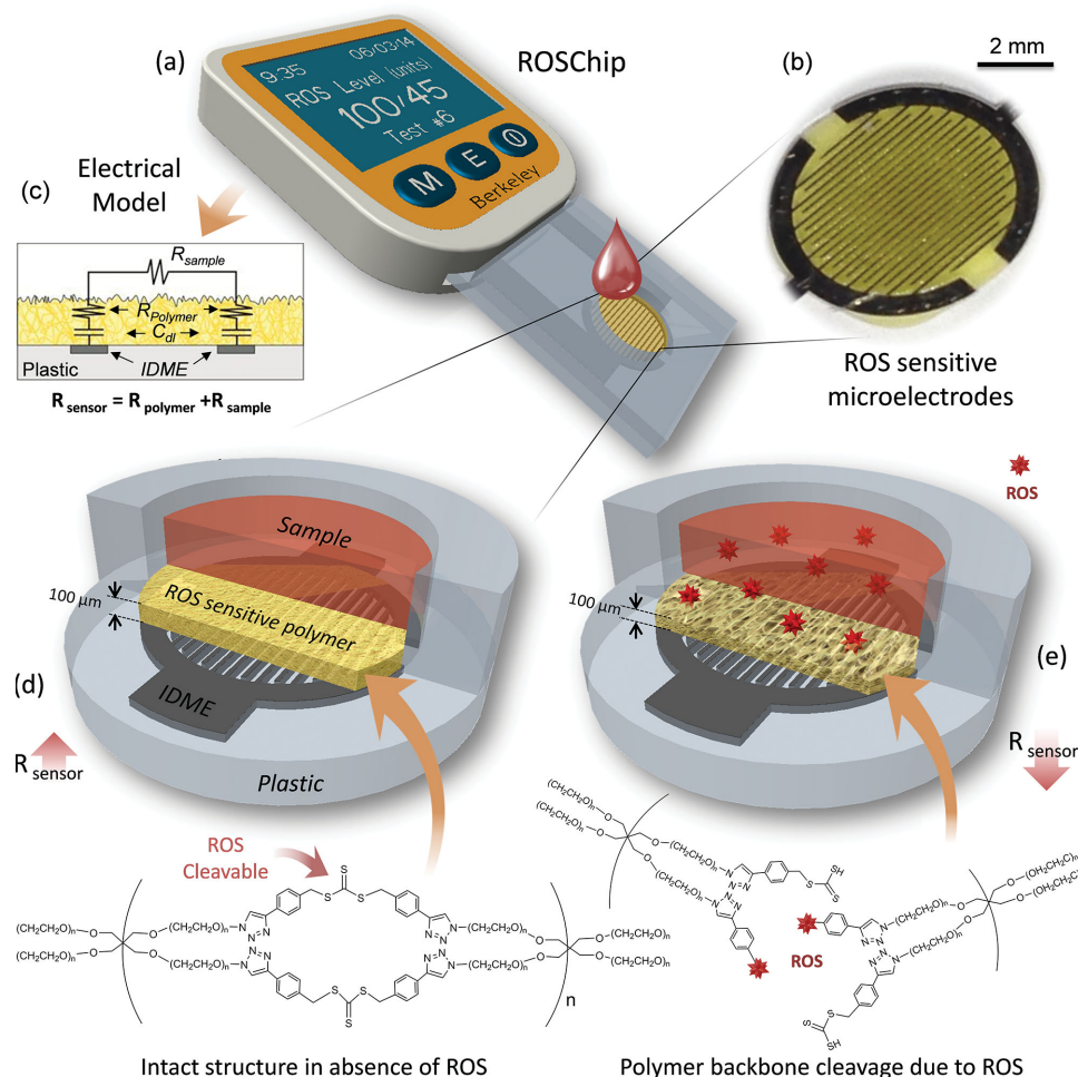
Figure 1. ROSChip is an oxidative stress point-of-care biosensor based on ROS-responsive electrodes. ROSChip is an electrode-based biosensor that is composed of interdigitated microelectrodes (IDMEs) coated with a thin film of a ROS-sensitive hydrogel polymer, termed RRG, that contains ROS-degradable thiocarbamate linkages in its backbone. The RRG acts as an electrical insulator, causing high resistance of the IDMEs in their initial state. However, exposure to radical oxidants present in the sample result in RRG degradation that decreases the IDMEs resistance that can be detected via a handheld voltage meter. a) ROSChip is a plastic cartridge designed for the POC monitoring of oxidative stress. b) A picture of IDMEs coated with the RRG. c) A simplified serial circuit to quantify ROSChip response. C_{dl} represents the capacitance behavior of the sensor that is directly associated with the RRG properties. R_{polymer} and R_{sample} represent the total resistance of the sensor ( R_{sensor} ). d) The RRG polymer remains intact in the absence of ROS, its electrical insulating properties are maintained and the total resistance of the sensor is high. e) The total resistance of the sensor reduces in the presence of ROS as the RRG thiocarbamate linkages break and the polymer degrades.
