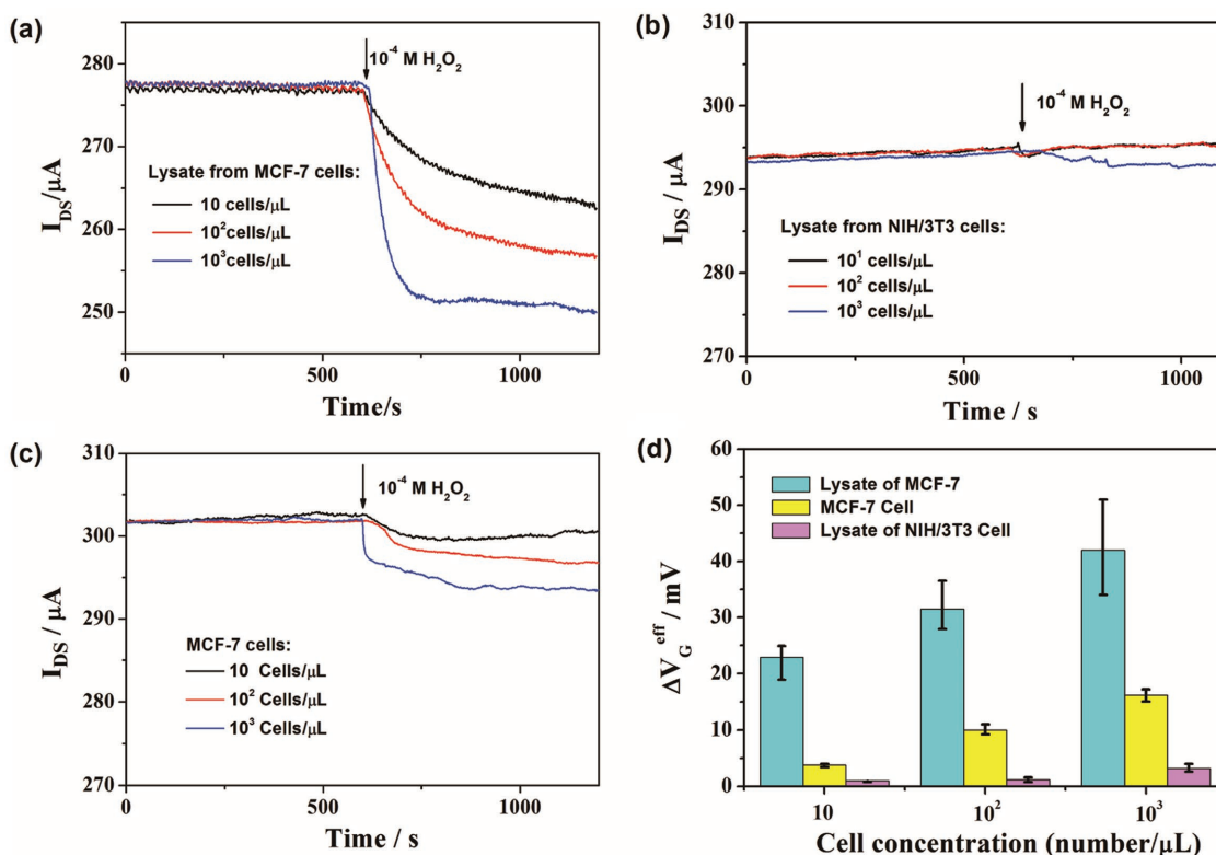
Figure 4. OECT-based protein sensors for the detection of cancer cells. a) Current responses of OECTs modified with the lysate of MCF-7 cancer cells to the additions of 10^{-4} M H_2O_2 . V_G = 0.6 V and V_{DS} = 0.05 V. b) Current responses of OECTs modified with the lysate of normal cells NIH/3T3 (control devices). c) Current responses of OECTs modified with MCF-7 cells on the gates. d) The change of the effective gate voltage \Delta V_G^{eff} for the devices modified with different cell lysates or whole cells. Error bars are calculated from at least 3 devices.
