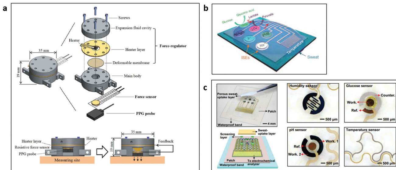
Figure 8. The use of add-ons for improving accuracy and stability. a) Integration of a force regulator with a PPG sensor contact force between the skin and a PPG sensor constantly for the consistent and stable PPG measurement results independent of body movements. Reproduced with permission. [277] Copyright 2018, AIP Publishing. b) Integration of a micro-sized RTD type temperature sensor next to several sensing modules to compensate measurement results depending on the temperature. Reproduced with permission. [75] Copyright 2016, Springer Nature. c) Integration of temperature, humidity and pH sensors to obtain more accurate glucose measurement results where the three additional elements were monolithically integrated with the glucose-sensing element on the flexible substrate. Reproduced with permission. [68] Copyright 2017, AAAS.
