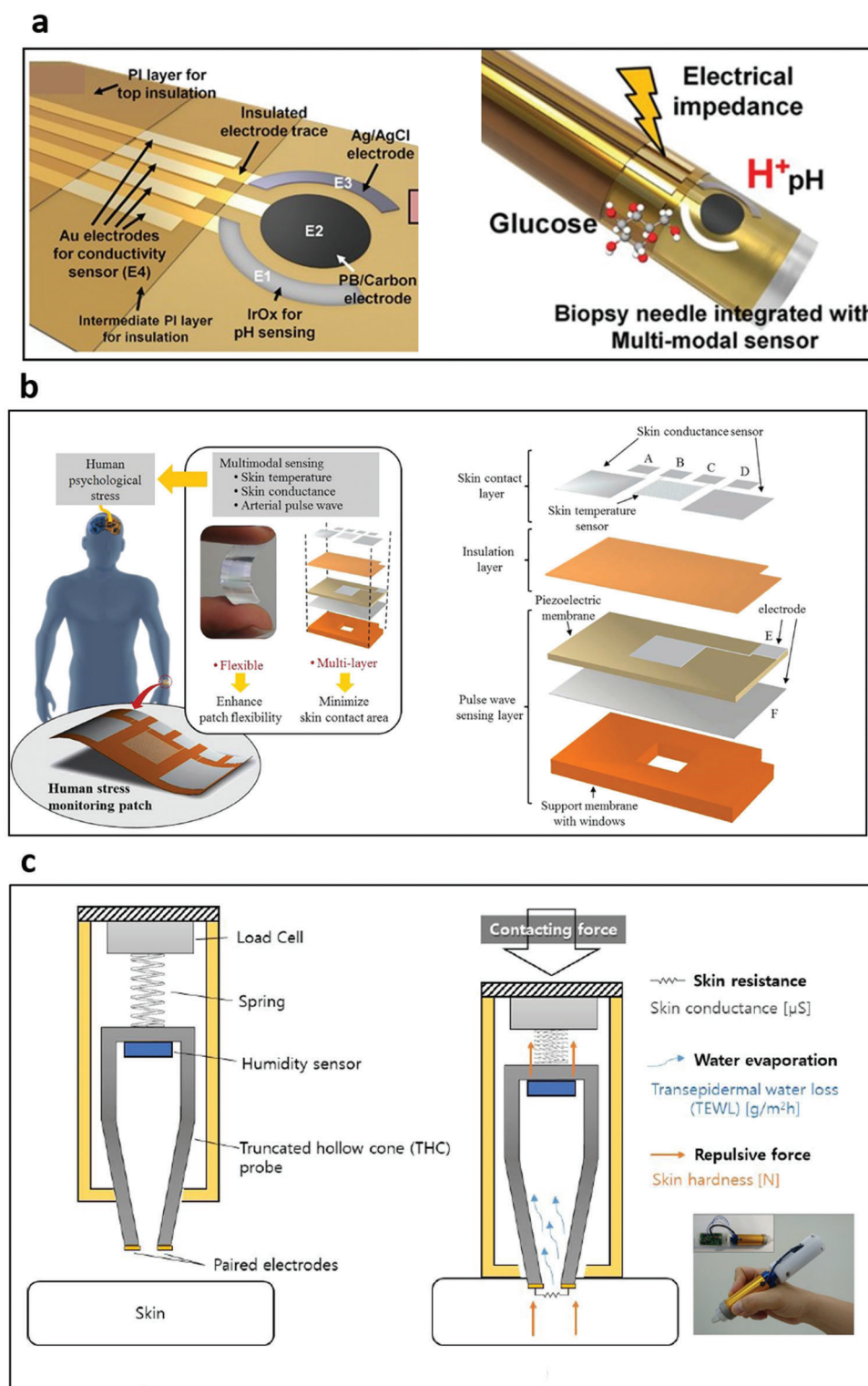
Figure 7. Integration designs of multimodal platforms for reducing measuring site. a) Physical/chemical sensor arrays where electrodes for a conductivity sensor were patterned in the middle of each electrode for glucose and pH sensing applications, showing the fabrication of the multimodal sensors placed on a surface of the small diameter needle. Reproduced with permission. [213] Copyright 2020, Elsevier. b) Reduced size of stress monitoring patch with a size comparable to that of a stamp, while measuring multiple physical biomarkers such as skin temperature, skin conductance and pulse wave. Reproduced with permission. [214] Copyright 2016, Springer Nature. c) Specific design of a probe that enabled three different biomarker measurements where the specially designed truncated hollow cone probe efficiently contained a force sensor above a conductance sensor with a sweat rate sensor placed inside the hollow probe. Reproduced with permission. [215] Copyright 2019, MDPI.
