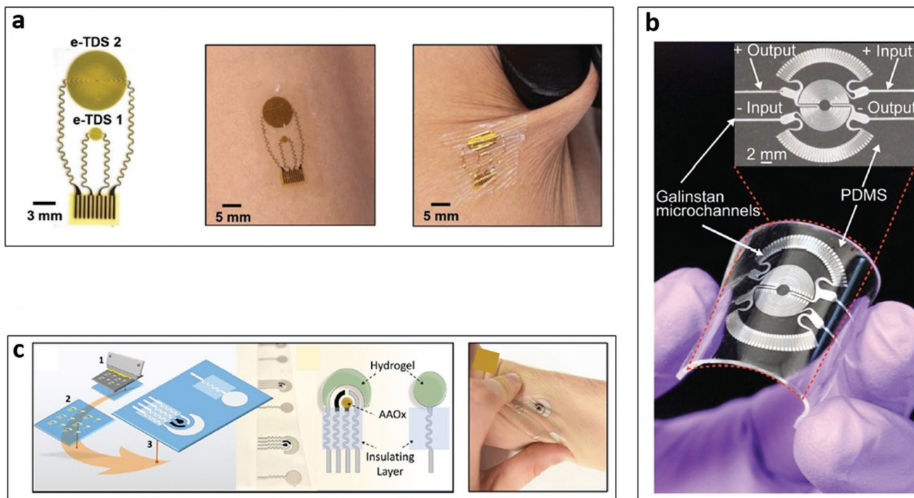
Figure 5. Flexible substrate-based biomarker sensing platforms. a) Epidermal electronic systems to measure thermal properties of human skin. Reproduced with permission. [173] Copyright 2018, Wiley-VCH. b) Physical biomarker sensors targeting pressure related to human skin by microfluidics-based diaphragm pressure sensor. Reproduced with permission. [187] Copyright 2017, Wiley-VCH. c) Tattoo-type sensors utilizing a sweat-based epidermal enzymatic biosensor for the assessment of Vitamin C levels. Reproduced with permission. [196] Copyright 2020, American Chemical Society.
