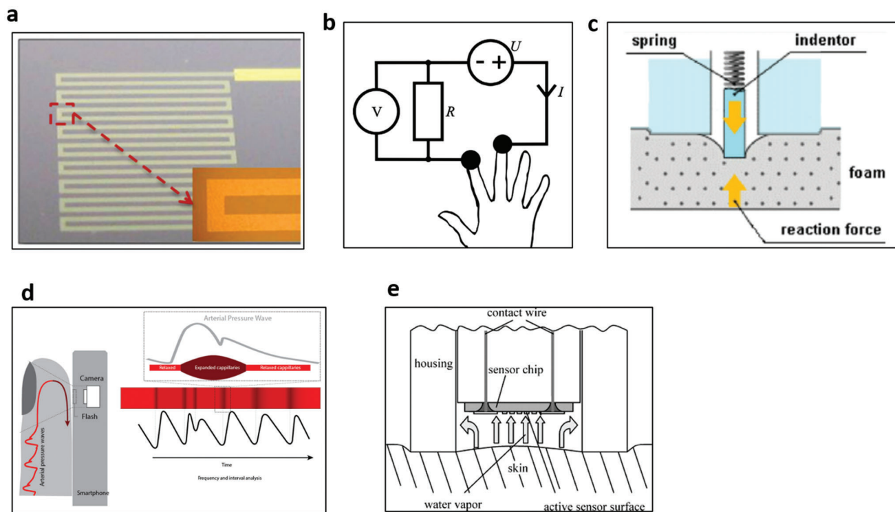
Figure 3. Physical sensing principles for measuring various biomarkers on skin. a) Resistance temperature detector (RTD) for skin temperature. Reproduced with permission. [92] Copyright 2012, IOP Publishing. b) 2-wire conductance measuring principle for skin conductance. Reproduced with permission. [102] Copyright 2013, Elsevier. c) Indentation method for skin hardness. Reproduced with permission. [105] Copyright 2006, IOP Publishing. d) Photoplethysmography (PPG) for pulse wave. Reproduced with permission. [106] Copyright 2017, JMIR Publication. e) Closed chamber method for sweat rate. Reproduced with permission. [110] Copyright 2008, Elsevier.
