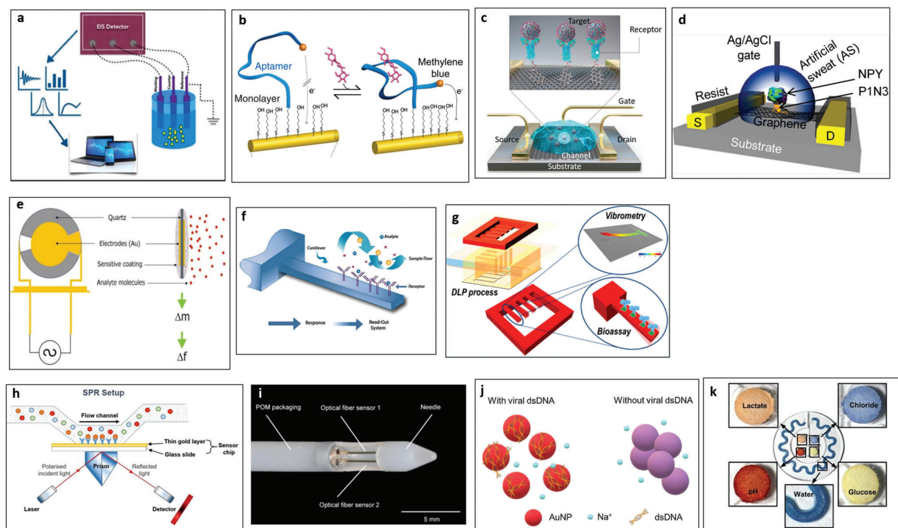
Figure 4. Transducers for biochemical sensing. a) Electrochemical impedance spectroscopy (EIS). Reproduced with permission. [114] Copyright 2018, MDPI. b) Sensing efficacy improvement using antifouling self-assembled monolayers for the real-time biomarker monitoring in an ambulatory rat. Reproduced with permission. [122] Copyright 2017, National Academy of Sciences. c) Field-effect transistors (FETs). Reproduced with permission. [127] Copyright 2020, American Chemical Society. d) Graphene-based FETs characterized in physiologically relevant environments (an artificial sweat with various ionic concentrations of the electrolyte). Reproduced with permission. [135] Copyright 2020, American Chemical Society. e) Quartz crystal microbalance (QCM). Reproduced with permission. [141] Copyright 2004, CIGR Journal. f) Cantilever. Reproduced with permission. [148] Copyright 2012, Elsevier. g) A 3D printed cantilever platform to overcome reproducibility and fabrication complexity issues. Reproduce with permission. Copyright 2017, American Chemical Society. h) Surface plasmon resonance (SPR). Reproduced with permission. [149] Copyright 2002, Springer Nature. i) A plasmonic sensing probe with tilted fiber Bragg grating imprinted on optical silica fibers. Reproduced with permission. [161] Copyright 2019, Elsevier. j) Colorimetric measurement. Reproduced with permission. [167] Copyright 2020, Elsevier. k) Microfluidic colorimetric detection reservoirs for the determination of multiple biomarker concentrations. Reproduced with permission. [164] Copyright 2016, AAAS.
