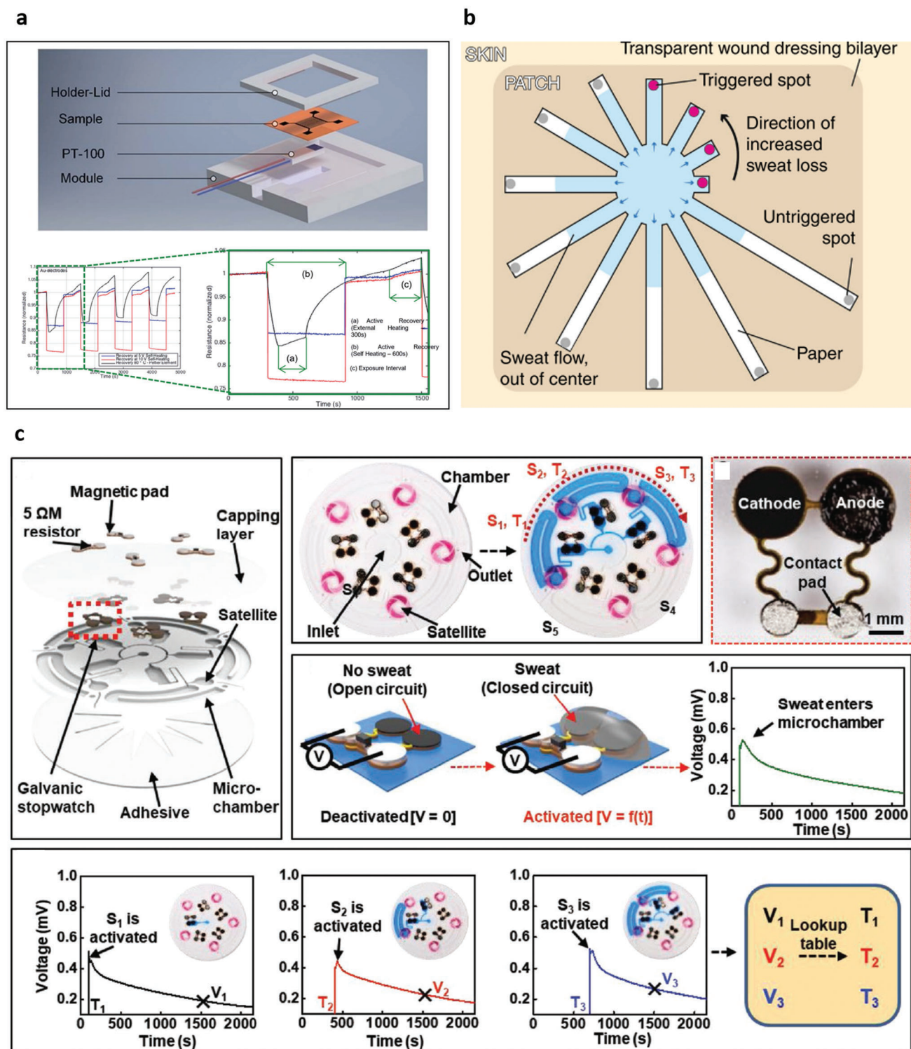
Figure 9. The strategies for improving sensor recovery time and continuous measurement. a) Self-recovering gas sensors by using CNTs as both the sensing element and heater, significantly improving baseline drift and response time. Reproduced with permission. [221] Copyright 2018, Royal Society of Chemistry. b) Paper-based microfluidic skin patches where channels are patterned and radially arranged with different lengths to realize the discrete real-time measurement of sweat secretion. Reproduced with permission. [226] Copyright 2019, Springer Nature. c) Sweat collection through microchannels where the passive valves were used for chronometric collection of sweat, resulting in time-dynamic analysis of sweat analysis using galvanic stopwatches. Reproduced with permission. [227] Copyright 2019, Wiley-VCH.
