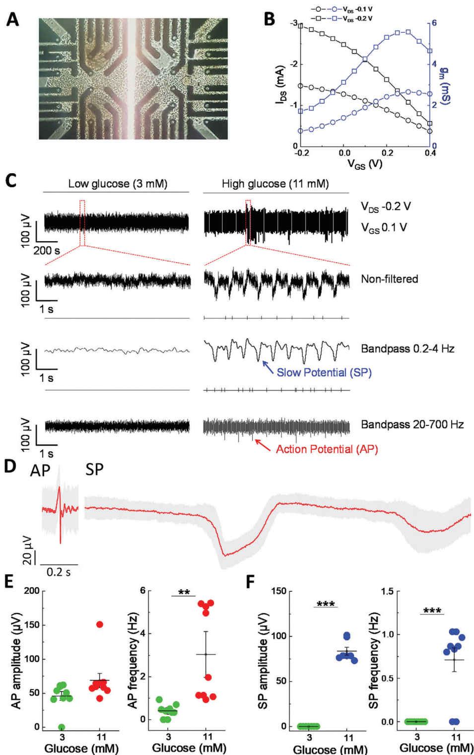
Figure 6. Recording of endocrine islet cells on vOECTs. A) vOECT Array with pancreatic islet cell clusters. B) Transfer and transconductance curves at V_{DS} = -0.1 and -0.2 V at V_{GS} = -0.2 to 0.4 V of vOECTs with islets in culture medium. C) Representative raw and filtered recordings of islets at low glucose (non-stimulatory, 3 mM) and high glucose (stimulatory, 11 mM) in physiological buffered ion solution at V_{DS} = -0.2 V and V_{GS} = 0.1 V. The different time scales are shown as well as non-filtered and band pass filtered traces (0.2–4 Hz, 20–700 Hz). The presence of slow potentials reflecting islet \beta -cell coupling are indicated. D) Average AP and SP at 15 mM glucose ( V_{DS} = -0.2 V, V_{GS} = 0.1 V; mean in red and SEM in gray; AP mean amplitude 69 \mu V, n = 303 ; SP mean amplitude 110 \mu V, n = 141 ). E,F) Action potential and slow potential amplitudes and frequencies at low glucose and high glucose stimulation ( V_{DS} = -0.2 V, V_{GS} = 0.1 V). Means \pm SEM; paired t -test; ** 2p < 0.01 , *** 2p < 0.001 ; N = 9 .
