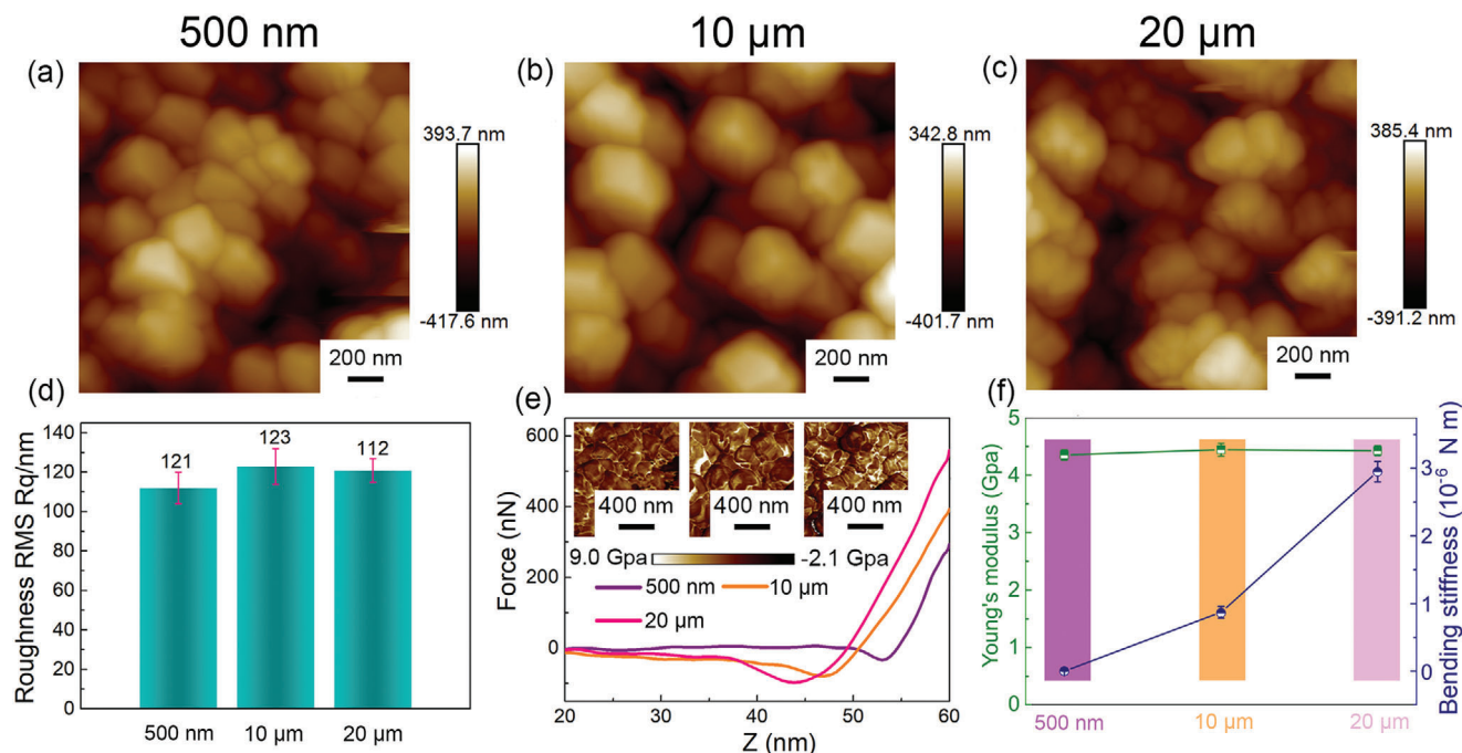
Figure 2. Morphology and tomography of the free-standing MOF films. AFM images of the free-standing MOF films with a) small thickness, b) mid thickness, and c) large thickness. d) The roughness of the free-standing MOF films with various thicknesses. e) The force-displacement curves of the free-standing MOF films with various thicknesses. Insets are mappings of DMT moduli of the free-standing MOF films with various thicknesses. f) The calculated Young's moduli and bending stiffnesses of the free-standing MOF films with various thicknesses.
