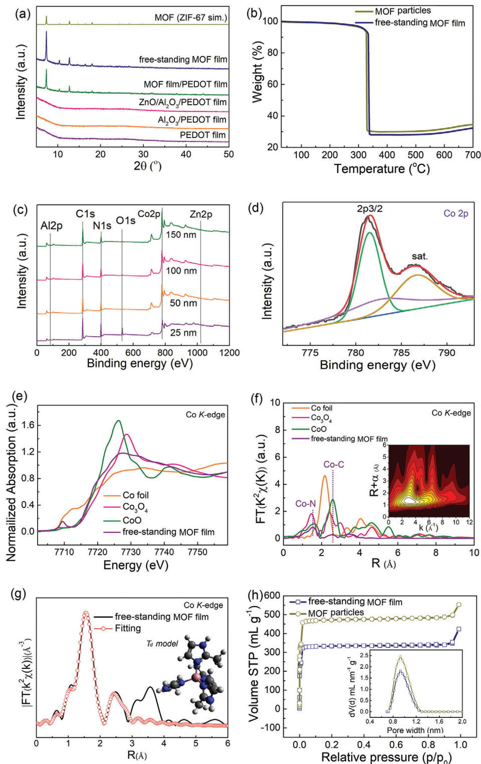
Figure 4. Structural characterizations of the free-standing MOF film. a) XRD patterns of PEDOT film, Al 2 O 3 /PEDOT film, ZnO/Al 2 O 3 /PEDOT film, MOF film/PEDOT film, and free-standing MOF film. Simulated patterns of MOF (ZIF-67 (sim.)) is also shown for comparison. b) TGA curve of free-standing MOF film compared with that of MOF particles. c) XPS survey scans at various depths of the free-standing MOF film. d) High resolution Co 2p 3/2 spectrum of the free-standing MOF film. e) XANES spectra and f) FT k 3 -weighted EXAFS spectra of the free-standing MOF film, CoO, Co 3 O 4 , and Co foil. Inset demonstrates a WT analysis of the free-standing MOF film. g) Fitting result of the FT-EXAFS for the free-standing MOF film at Co K-edge. Inset of (g) shows a T d model of ZIF-67 structure. h) Nitrogen adsorption-desorption isotherms of the free-standing MOF film and the MOF particles. Inset demonstrates the corresponding pore size distributions.
