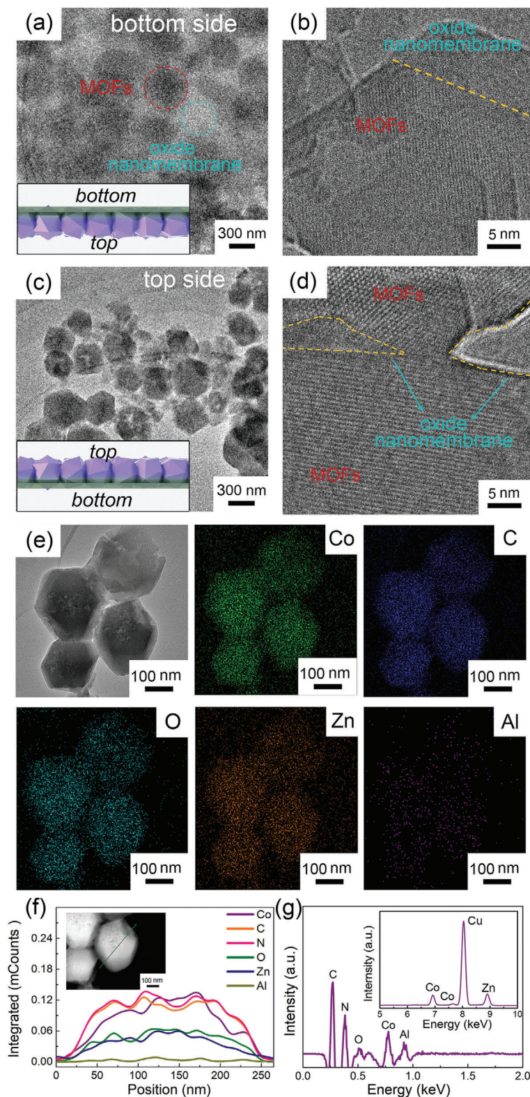
Figure 3. Formation mechanism of the free-standing MOF film. a) and b) Cryo-TEM images of free-standing MOF film (bottom side view) with low and high magnifications. The inset is corresponding schematics. c) and d) Cryo-TEM images of free-standing MOF film (top side view) with low and high magnifications. The inset is corresponding schematics. e) Cryo-TEM image of the free-standing MOF film with elemental mapping results. f) Linear EDS scan along the dashed line in the inset, demonstrating the distribution of the elements in the free-standing MOF film. Inset is the TEM image with high magnification. g) EDS spectrum of the free-standing MOF film in (e). The inset is the high energy region of the spectrum.
