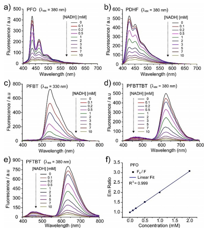
Figure 2. Fluorescence response of polyfluorene Pdots to NADH. (a–e) Emission spectra of polyfluorene Pdots at 0–10 mM NADH with excitation of the fluorene group ( \lambda_{\text{ex}} = 330 or 380 nm). Pdot emission intensity decreases with increasing NADH. (f) Stern–Volmer plot for PFO Pdots showing the ratio of fluorescence emission intensity at 428 nm in the absence ( F_0 ) and presence ( F ) of NADH at various NADH concentrations ( \lambda_{\text{em}} = 436 nm). F_0/F showed a linear relationship with NADH concentration over the physiological range of 0–2 mM NADH.
