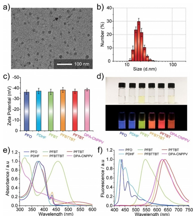
Figure 1. Characterization of Pdots. (a) TEM image of PFBT Pdots. (b) Size distribution of PFBT Pdots based on DLS measurements. (c) Zeta potentials of six Pdots. (d) Photographs of Pdot suspensions illuminated by ambient indoor light (upper) and UV light (365 nm; lower). Pdot emissions are intense and span the visible spectrum. (e) Absorption spectra. (f) Emission spectra ( \lambda_{\text{ex}} = 365 nm).
