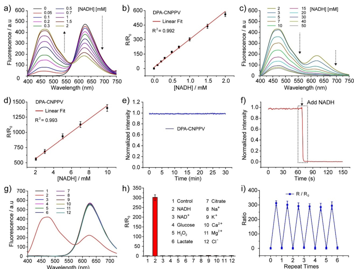
Figure 3. Reversible ratiometric NADH sensing using DPA-CNPPV Pdts. (a) Emission spectra of DPA-CNPPV Pdts ( 0.02 \text{ mg mL}^{-1} ) at 0–2 mM NADH with excitation at 385 nm. (b) Ratiometric calibration curve, calculated using data shown in panel a. R = I_{458\text{nm}}/I_{627\text{nm}} ; R_0 = R in the absence of NADH. (c) Emission spectra of DPA-CNPPV Pdts at 2–50 mM NADH, and (d) corresponding ratiometric calibration curve. (e) Photostability of DPA-CNPPV Pdts indicated by consistent emission at 627 nm for 30 min with excitation at 385 nm. (f) Rapid response ( < 5 \text{ s} ) of DPA-CNPPV Pdts to addition of 1 mM NADH. (g) Emission spectra of DPA-CNPPV Pdts in the presence of NADH (red curve), 10 other analytes, and a PBS control, demonstrating the specificity of the response to NADH. Numbers 1–12 are defined in panel h. (h) Selectivity of DPA-CNPPV Pdot response to NADH versus 10 other biological analytes at 1 mM. R/R_0 values were calculated based on the spectra shown in panel g. Only NADH (red bar) produced a significant fluorescence response. (i) Reversibility of response of DPA-CNPPV Pdts to repeated exposure to 0 and 1 mM NADH DPA by using ultrafiltration and gel filtration.
