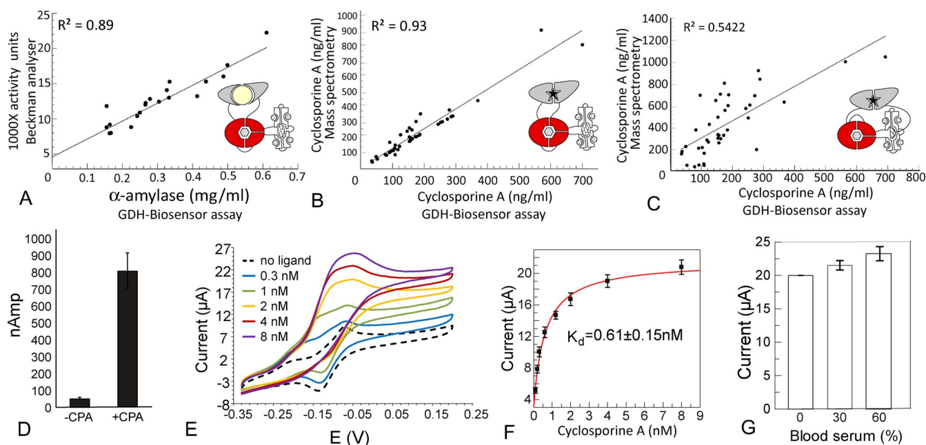
Figure 4. Quantification of biomarkers in human fluid samples using assays based on cpGDH-CaM biosensors. A) Detection of \alpha -amylase in human saliva \alpha -amylase biosensor (X-axis) and its comparison with the clinical \alpha -amylase activity assay (Y-axis). B) Quantification of Cyclosporine A in blood of kidney transplant patients using cpGDH-CaM biosensor-based assay (X-axis) and its comparison with the clinical Cyclosporine A LC-MS assay (Y-axis). C) The blood samples from B were retested using the assay based on a two component GDH biosensors of Cyclosporine A. [12] D) Electrochemical response of 200 nM single component Cyclosporine A (CPA) sensor to absence and presence of 250 nM Cyclosporine a (average of n=3 plotted, error bars are SD). Sensor enzymatic activity is reported as maximum nA increase per minute using disposable DropSense gold electrode polarized at +0.1 V vs. Ag reference strip and 1-methoxy-5-methyl phenazinium methylsulfate as an electron mediator. E) Typical cyclic voltammograms of GDH-CaM- Cyclosporine A functionalized gold electrode upon exposure to different concentrations of Cyclosporine A. The potential scan rate was 2 \text{ mV s}^{-1} ; the potentials were measured vs. Ag/AgCl/3MKCl reference electrode. F) A plot of values obtained in three independent replicates of the experiment shown in (E). The data was fit to a quadratic equation leading to a K_d value of 0.6 nM. G) Analysis of the impact of the serum addition to the sample on the performance of GDH-CaM-Cyclosporine A biosensor functionalized bioelectrode. In the experiment, the electrode was activated by addition of 10 nM of Cyclosporine A to a sample containing indicated concentrations of human serum.
