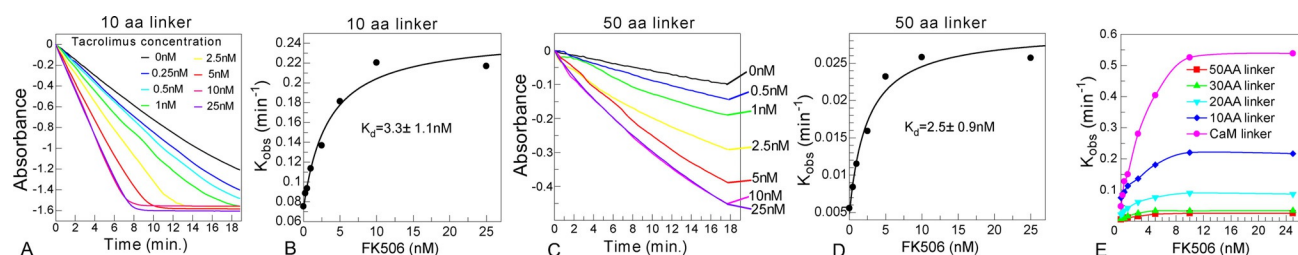
Figure 2. Response of circularly permuted (cp)GDH-tacrolimus biosensors with different linker lengths, plotted against increasing concentration of the drug. A) GDH activity of 10 nM solution of calcineurin A/B-cpGDH-FKBP fusion carrying 5 GS repeats between S403 and N405 in the presence of increasing concentrations of tacrolimus. The activity of the enzyme was monitored by changes in absorption of 60 \mu M electron accepting dye dichlorophenolindophenol in the presence of 0.6 mM electron mediator phenazine methosulphate, 20 mM of glucose, 1 \mu M PQQ and 1 mM \text{CaCl}_2 . B) The fit of the data shown in A leading to a K_d value of 3.3 nM. C) GDH activity of 10 nM solution of CaA/CaB-cpGDH-FKBP fusion carrying 50 amino acid linker. D) The fit of the data shown in (C) leading to a K_d value of 2.5 nM. E) Comparison of dynamic ranges of (cp)GDH-tacrolimus biosensors developed in this study.
