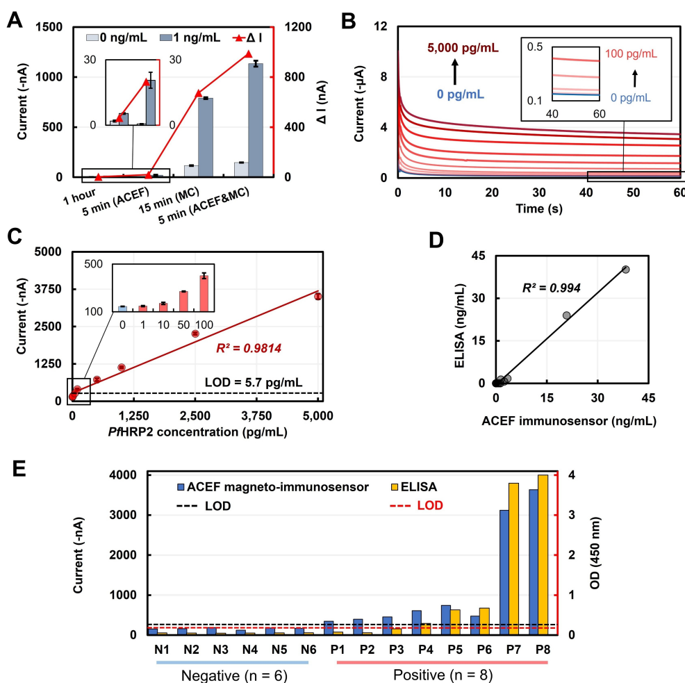
Figure 4. Performance of the ACEF-enhanced magneto-immunosensor for quantifying Pf HRP2 in spiked and clinical blood samples.
