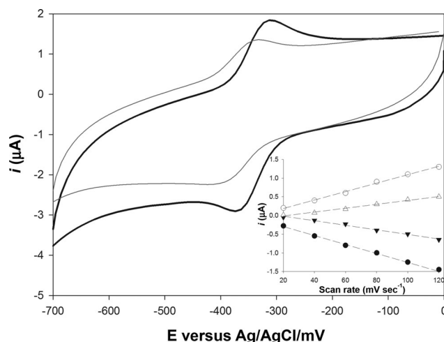
FIG. 2 Anaerobic cyclic voltammograms of GOD on DDAB glassy carbon electrodes in the absence (thin line) and in the presence (bold line) of GO. Scan rate: 120 \text{ mV s}^{-1} . Inset: plot of cathodic (filled symbols) and anodic (empty symbols) peak currents versus scan rate for GOD on DDAB glassy carbon electrodes in the absence (triangles) and in the presence (circles) of GO. R^2 > 0.99 .
