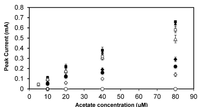
Figure 2. Correlation of peak current with the acetate concentration added for different HCF(III) concentrations in the marine MFC biosensor. Concentrations of HCF(III) (mM) were 0.8 (squares), 0.4 (triangles) 0.2 (diamonds) and 0 (spheres). Dissolved oxygen was > 6 (open symbols) and 0 mg/L (closed symbols). Results show averages of triplicate measurements.
