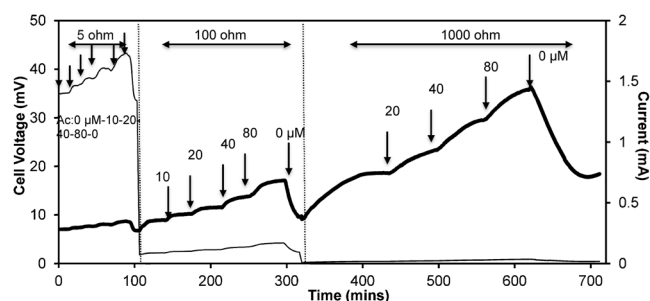
Figure 6. Cell voltage (thick line) and current (thin line) responses of the marine MFC biosensor to step changes in acetate concentration of the inflow under continuous flow mode. Small resistors (5 Ω) and large resistors (1000 Ω) amplify the current and cell voltage signals respectively.
