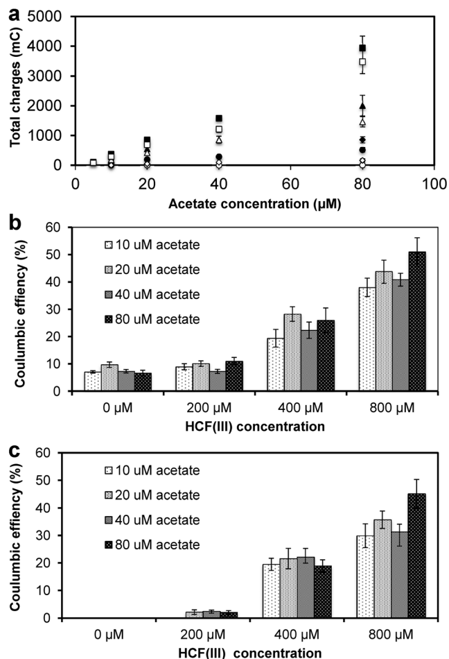
Figure 3. Effect of added HCF(III) concentrations on (a) total produced coulombic, charges coulombic efficiencies of the marine MFC biosensor in the absence (b) and presence (c) of dissolved oxygen. Results are the averages of triplicates. Concentrations of HCF(III) (mM) were 0.8 (squares), 0.4 (triangles) 0.2 (diamonds) and 0 (spheres). Dissolved oxygen was > 6 (open symbols) and 0 mg/L (closed symbols).
