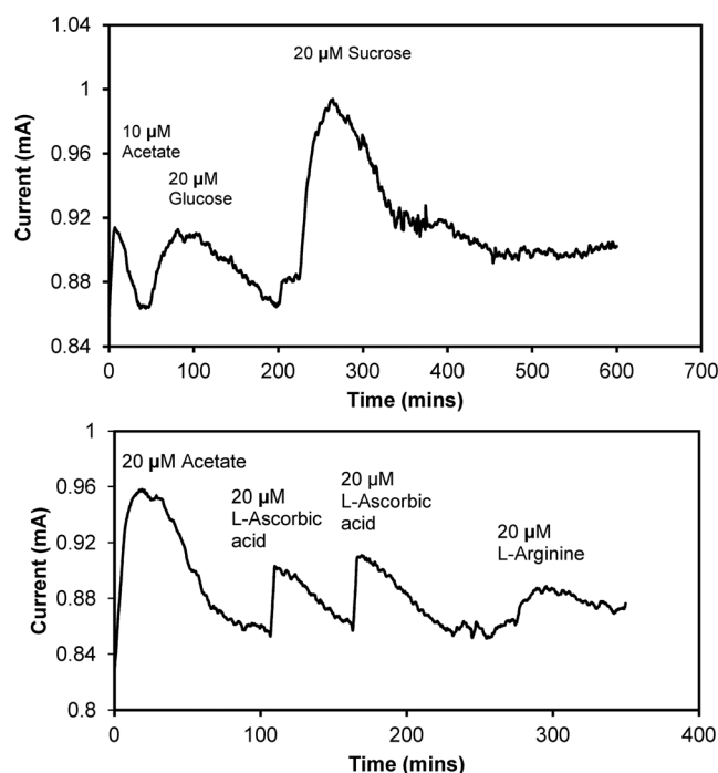
Figure 4. Response of acetate adapted marine MFC biosensor to more complex organic substances (DO > 6 mg/L, HCF(III) = 0.4 mM, external resistance = 5 ohm)
