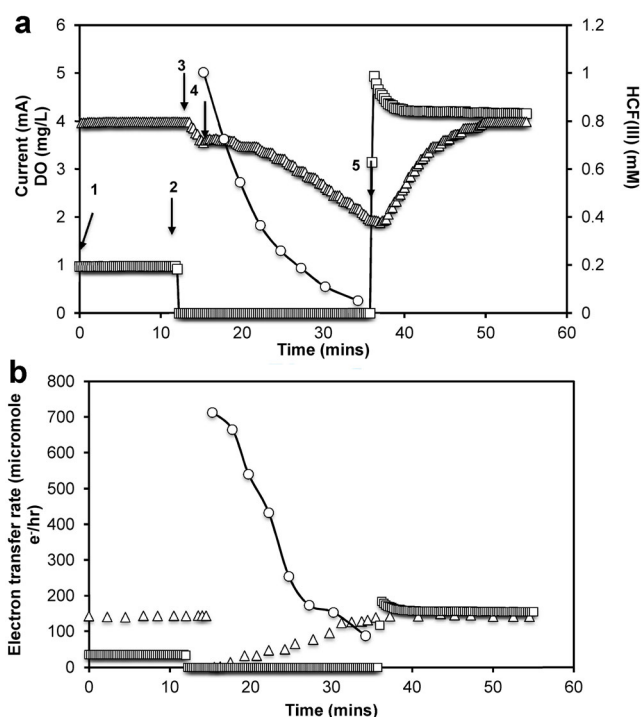
Figure 5. Effect of HCF(III) addition to the acetate saturated marine MFC biosensor on biofilm oxygen uptake and current production. (a) Profiles of DO (triangle), current (square) and HCF(III) concentration (circle). Arrows indicate: ① 5 Ω and aeration, ② 1 MΩ, ③ aeration stopped, ④ addition of 1 mM HCF(III), ⑤ 5 Ω and aeration. (b) Electron transfer rates to HCF(III) (circle), oxygen (triangle) and anode (square).
