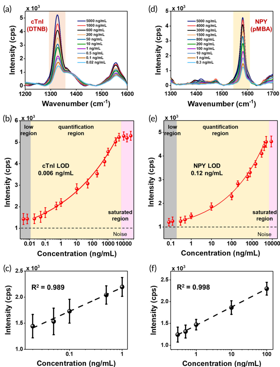
FIGURE 3 cTnI and NPY detection with PRADA. (a) Raman spectra of cTnI in human serum and (b) SERS intensity at the characteristic DTNB peak ( 1,325\text{ cm}^{-1} ) as a function of cTnI concentrations. The low region (gray box) was where the concentrations were below the detection limit; quantification region (yellow box) was used to determine LOD with a 4PL function fit; and saturated region (pink box) was where high density of analytes saturated PRADA. (c) Linear fit of the DTNB peak at low concentrations of cTnI in the range of 0.02 to 1 ng/mL. (d) Raman spectra of NPY in human serum by monitoring the pMBA peak at 1580\text{ cm}^{-1} . (e) SERS intensity at the characteristic pMBA peak as a function of NPY concentrations. (f) Linear fit of the pMBA peak at low concentrations of NPY ranging from 0.3 to 100 ng/mL. Error bars indicate the standard deviations from at least five measurements. A base 10 logarithmic scale was used for x-axis. 4PL, four-parameter logistic; LOD, limit of detection; PRADA, portable reusable accurate diagnostics with nanostar antennas; SERS, surface enhanced Raman spectroscopy
