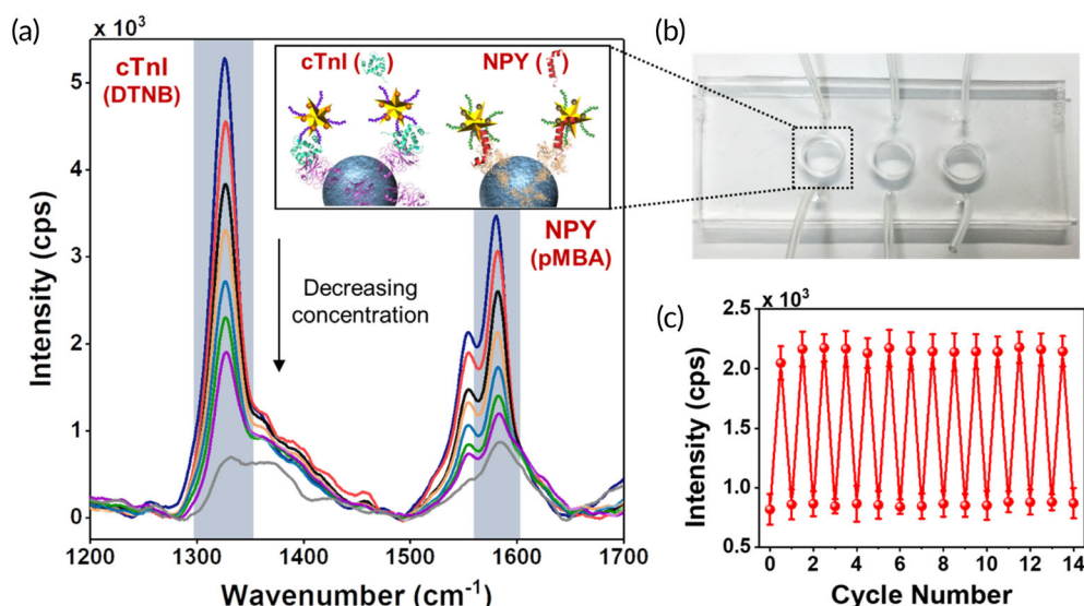
FIGURE 4 Multiplexing and reusability with PRADA. (a) Multiplexed detection of both cTnI and NPY in a three-well microfluidic device. The concentrations measured in ng/ml for cTnI/NTNB are 3000/1500 (blue), 1000/600 (red), 400/200 (black), 200/100 (orange), 5/10 (light blue), 0.5/1 (green), 0.05/0.3 (purple), and control (gray). The inset is a schematic representation of multiplexed detection of both biomarkers. (b) Image of a microfluidic device utilized in the experiments. (c) Demonstration of reusability of PRADA where the same microfluidic chip was reused 14 times after washing and regenerating. Here, 0.1 ng/ml of cTnI was detected at the DTNB Raman peak with minimal signal loss. Error bars indicate the standard deviations from at least five measurements. PRADA, portable reusable accurate diagnostics with nanostar antennas
