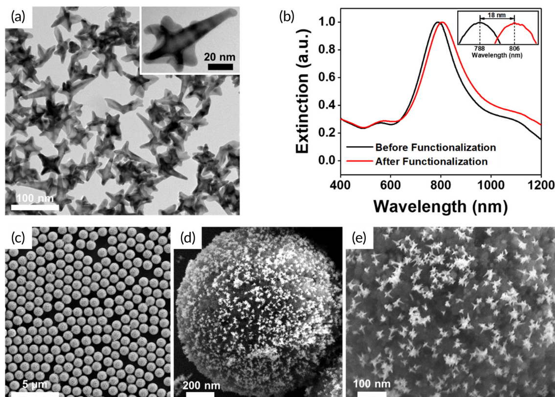
FIGURE 2 Characterization of PRADA. (a) Transmission electron micrograph of GNSs showing their anisotropic morphology. (b) Extinction spectra of bare GNSs and GNSs functionalized with SERS barcodes and peptide BREs. (c–e) SEM images of complete immunocomplexes at various magnifications with magnetic beads capture probes and GNS-SERS barcodes detection probes. BREs, biorecognition elements; GNSs, gold nanostars; PRADA, portable reusable accurate diagnostics with nanostar antennas; SEM, scanning electron micrograph; SERS, surface enhanced Raman spectroscopy
