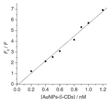
Figure 9. Stern–Volmer plot of F_0/F versus [\text{AuNPs-}\beta\text{-CDs}] . The linear approximation gives F_0/F = -0.13 + 5.8 [\text{AuNPs-}\beta\text{-CDs}] , R = 0.9955 .
