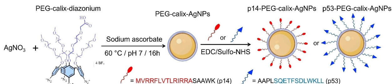
Scheme 1. Preparation of the peptide-AgNPs conjugates. Amino acids sequences of the p53-peptide and the p14-peptide necessary for the interaction with Mdm2 are labelled in blue or red respectively.
