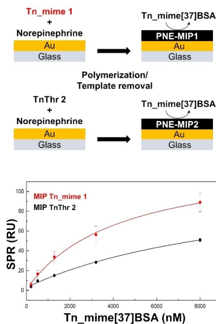
Figure 3. SPR analysis of Tn_mime[37]BSA affinity for PNE-MIP. Schematic representation of PNE imprinting and MIP formation for TnThr mimetic 1 and natural TnThr 2 (upper panel). SPR signals (mean \pm SD, n = 3 ) and binding curves (1:1 fitting) for Tn_mime[37]BSA SPR from serial dilution (dilution factor 2.5) of Tn_mime[37]BSA from 0.205 \mu M to 8.00 \mu M onto PNE-MIP surfaces 1 and 2 (lower panel). SPR sensorgrams are reported in Figure S2 (see Supporting Information).
