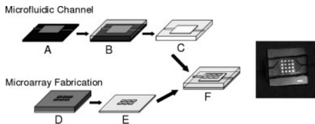
Figure 2. Schematic of the overall microfluidic chip assembly process showing the steps from the patterns of the microfluidic channels and grid to the finished SF10 glass chip: (A) SU-8 photoresist is patterned to make a silicon mold; (B) PDMS is poured on silicon mold and allowed to set; (C) PDMS replica with microchannels, (D) photolithography on SF10 glass chip; (E) gold evaporation and lift off; (F) PDMS chip is bound over the gold spot array using a Corona etcher. The constructed microfluidic chip (right).
