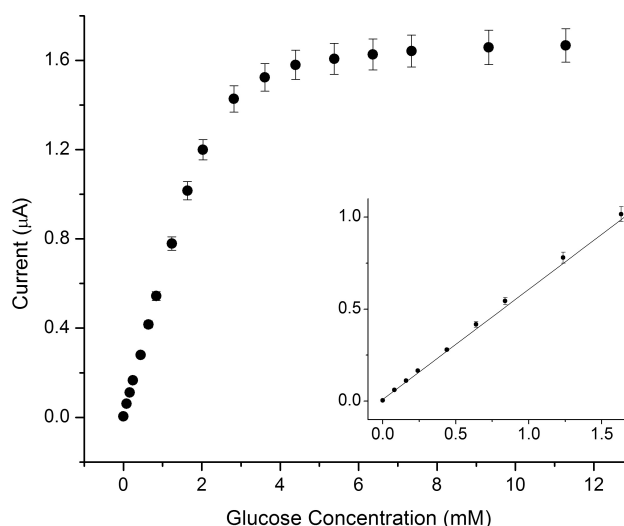
Fig. 6. A calibration curve for glucose biosensor. The inset plot shows the lower analyte concentration range. Error bars: standard error of the mean.
