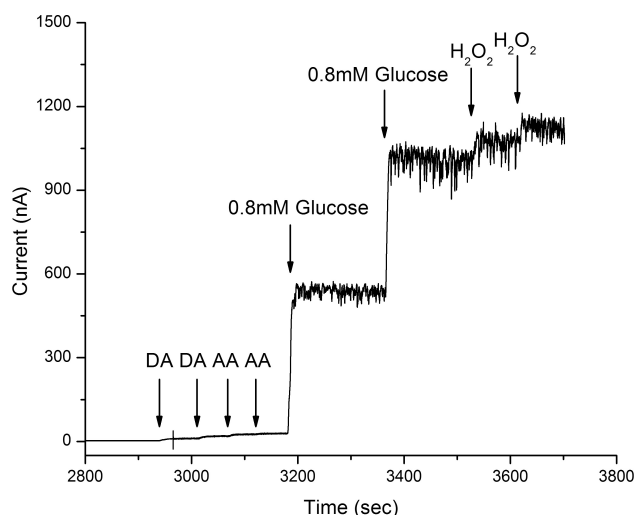
Fig. 4. Current responses of the glucose biosensor to interferents, glucose, and \text{H}_2\text{O}_2 . The biosensor response at a constant potential of 0.7 V (vs. Ag/AgCl) was monitored in stirred PBS solution upon sequential injections to give 5 and 10 \mu\text{M} of dopamine (DA), followed by 250 and 500 \mu\text{M} of ascorbic acid (AA), 0.8 and 1.6 mM of glucose (Glu), and 20 \mu\text{M} and 40 \mu\text{M} of hydrogen peroxide ( \text{H}_2\text{O}_2 ).
