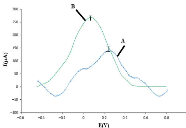
FIGURE 2 Cyclic voltammogram during different stages of address layer, (a) bare graphite electrode, (b) graphite/nanofiber modified electrode at the presence of B-R buffer with pH = 5 and 30 \mu M T_2 toxin. (Scan speed conditions = 100 mV/s.)
