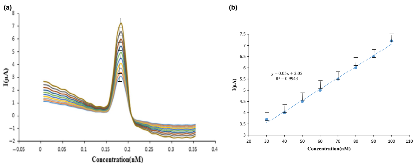
FIGURE 7 (a) Differential pulse voltammetry (DPV) techniques of the electrochemical behavior of T_2 toxin over the concentration range 30–100 nM at the presence of B-R buffer with pH = 5, (b) linear chart of the effect of different concentrations on the transition flow with compressibility coefficient = 0.99
