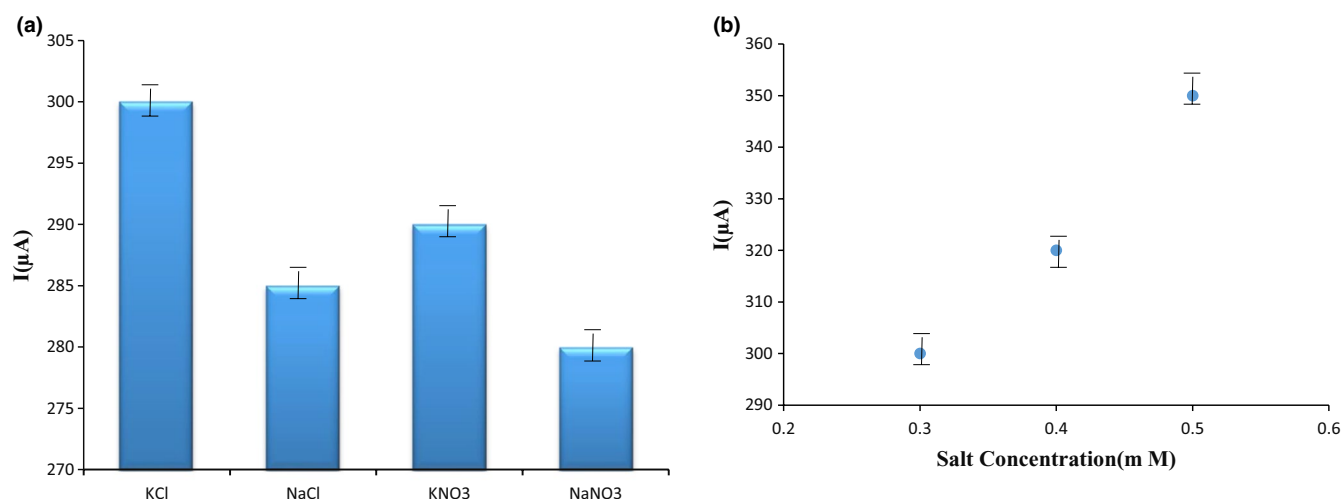
FIGURE 6 (a) The impact of different salt concentrations with 30 \mu\text{M} T_2 toxin on the surface of the G/PAN nanofiber modified electrode to determine the effective salt concentration in electron transfer, (b) the effect of different concentrations of \text{KNO}_3 with 30 \mu\text{M} T_2 toxin on the surface of the G/PAN nanofiber modified electrode to recognize the effective salt concentration in electron transfer as a supporter electrolyte
