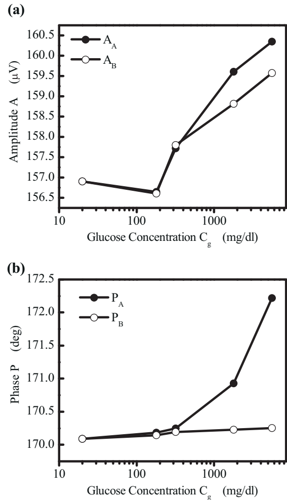
Figure 7 Single laser (laser A and laser B) PTR signals from serum-glucose solutions with glucose concentration from 20 mg/dl to 5600 mg/dl. (a) amplitude; (b) phase.
