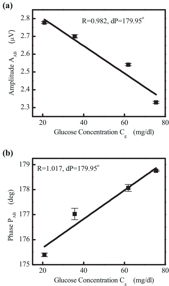
Figure 6 Optimal R - dP combinations for linear WM-DPTR signal response to glucose in the low glucose concentration range from 20 mg/dl to 80 mg/dl. (a) amplitude; (b) phase.
