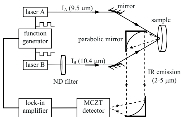
Figure 1 WM-DPTR system setup for glucose measurement. Square-wave modulated radiation from laser A ( 9.5\ \mu\text{m} ) and laser B ( 10.4\ \mu\text{m} ) co-incident on the sample generate superposed IR emissions. The differential infrared photon flux is collected by the MCZT detector acting as a band pass filter ( 2\text{--}5\ \mu\text{m} , dashed line) and sent to a lock-in amplifier. The function generator controls the phase shift between the two laser beams, and the variable circular neutral density (ND) filter controls the intensity ratio of the two lasers I_A/I_B .
