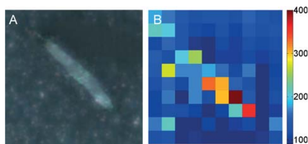
Figure 3 Bright-field image of a diatom frustule (A) and Raman mapping image of free DTNB (B) on a single diatom frustule.
