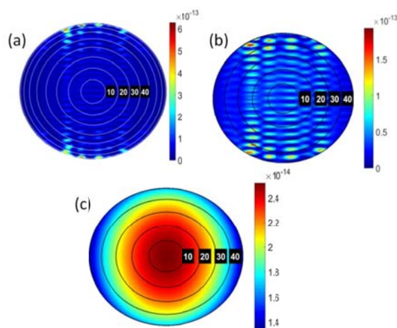
Figure 2. Far-field radiation pattern of fluorophore on diatom (a), and radiation pattern inside the 50^\circ solid angle on diatom (b) and glass (c).
