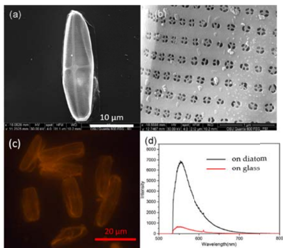
Figure 4. SEM images of (a) an overview of a single diatom frustule, (b) primary pores on a frustule, (c) fluorescence image of 1 \mu\text{L} of R6G ( 10^{-6} M) dropped onto the glass-diatom substrate, (d) fluorescence spectra of 1 \mu\text{L} of R6G ( 10^{-6} M) solution dropped onto the glass-diatom substrate.
