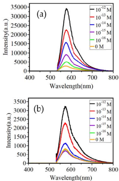
Figure 5. Fluorescence spectra on diatom (a) and glass (b) for different concentrations of IgG.
