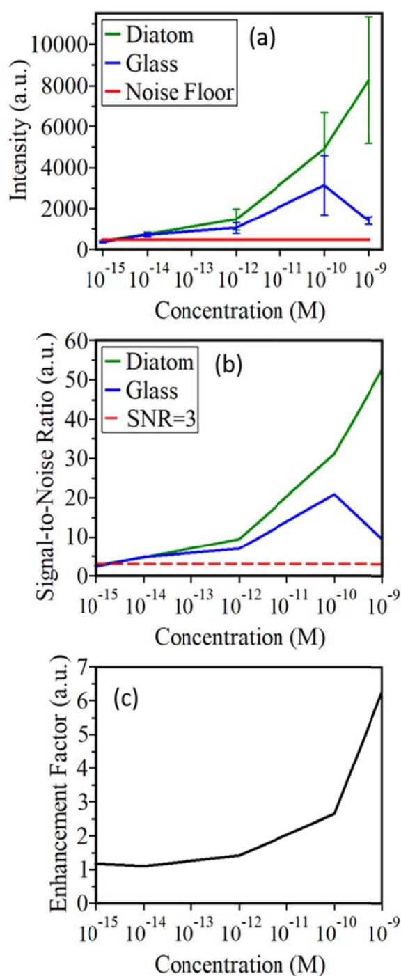
Figure 7. Average fluorescence on diatom and glass with error bars, along with the noise floor (a). The SNR is shown for diatom and glass with respect to concentration with a line representing \text{SNR} = 3 (b). The enhancement factor is also calculated at each concentration (c).
