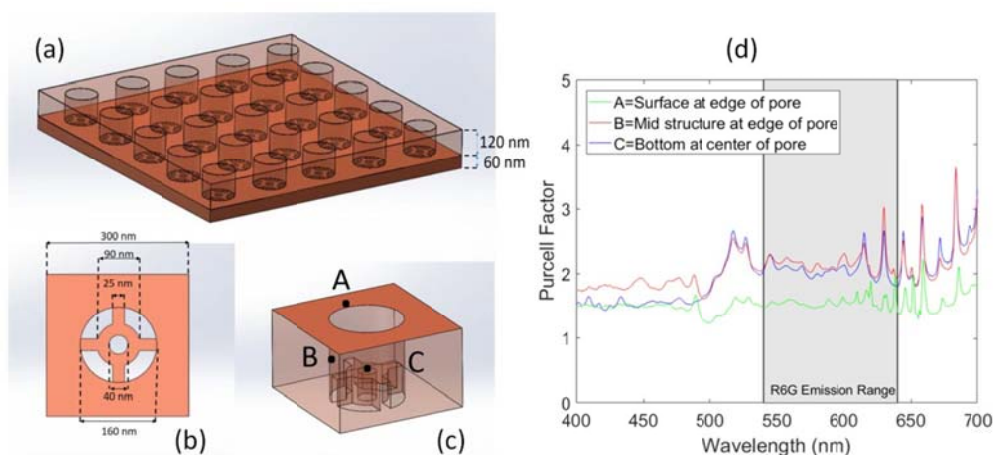
Figure 1. (a) Simulated slab structure with 5 \times 5 array of nanopores; (b) enlarged view of the nanopore with geometric parameters; (c) placement of fluorophores in diatom frustules; (d) the Purcell effect simulation results at the three points within a unit cell as a function of the wavelength
